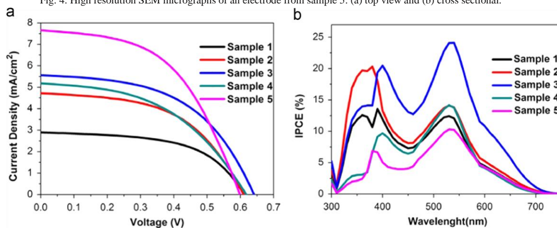
Fig. 5. (a) JV curve and (b) IPCE spectra for the five samples.
