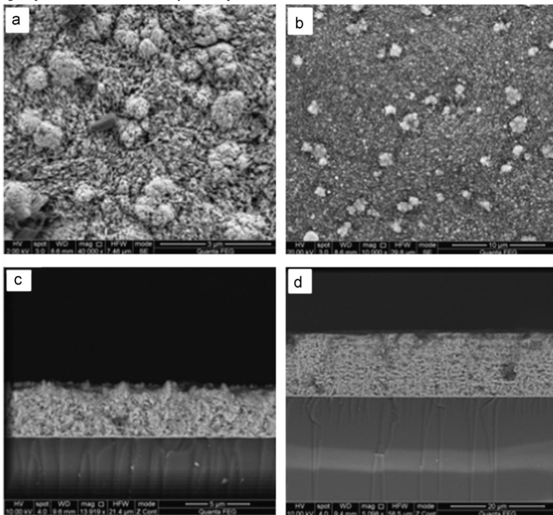
Fig. 3. SEM micrographs of electrodes from: (a) sample 4 - top view; (b) sample 5 - top view; (c) sample 4 - cross sectional view; and (d) sample 5 - cross sectional view.
