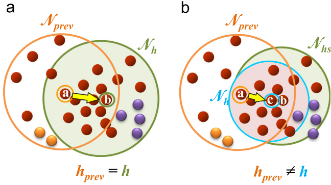
Fig. 4. The iteration in (a) uses a fixed h . Yellow arrow is a mean shift vector. Shifting windows in (b) are adjusted by our scale-adaptive method. The adjustment of \mathcal{N}_{prev} to \mathcal{N}_{hs} is based on the mean shift vector and center point's spatial scale \varphi_s , after which adjustment of \mathcal{N}_{hs} to \mathcal{N}_h is controlled by label variances inside \mathcal{N}_{prev} and \mathcal{N}_{hs} . In the second adjustment, the center of mass slightly shifts from b to c . (For interpretation of the references to color in this figure caption, the reader is referred to the web version of this paper.)
