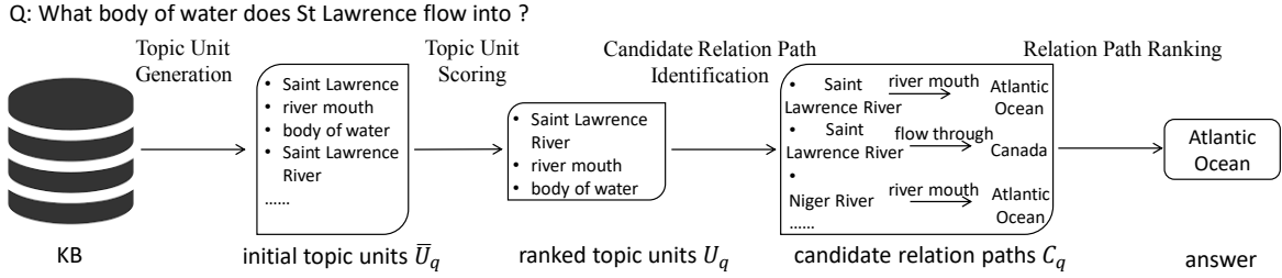
Figure 2: An overview of the various steps of our method.
