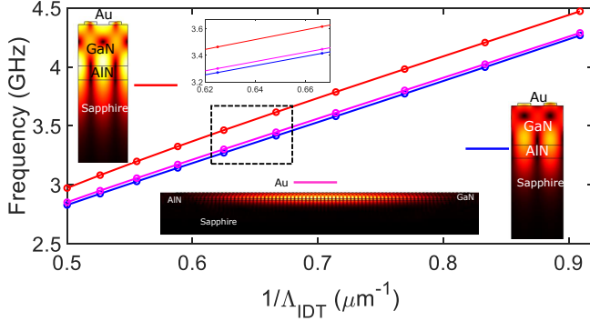
FIG. 3. Simulated frequencies of the two non-degenerate higher order Lamb wave modes (blue, inset right and red, inset left) as a function of inverse electrode period 1/\Lambda_{IDT} . The respective mode displacement profiles for the two modes are shown in the inset. The Lamb wave resonance (inset, bottom) frequency ( N_{pairs} = 40 ) is also shown (magenta). A zoomed-in section (shown by the dashed box) of the plot is shown in the inset for visualization. Simulation parameters: t_{GaN} = 1.5 \mu m , t_{AlN} = 0.35 \mu m and t_{Au} = 75 \text{ nm}
