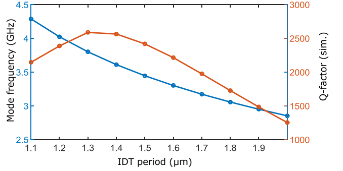
FIG. 4. Simulated Lamb wave fundamental resonance mode frequency (blue) and quality factor (brown) for GaN-on-sapphire devices with varying IDT periods ( N_{pairs} = 40 ). Simulation parameters: t_{GaN} = 1.5 \mu m , t_{AlN} = 0.35 \mu m and t_{Au} = 75 \text{ nm} .
