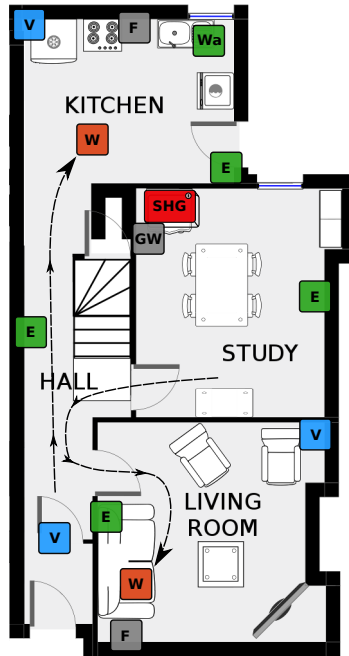
Figure 1: SPHERE device layout in the first floor of a residential house. SHG – the SPHERE Home Gateway. W – mobile wearables. V – video cameras with the attached video gateways. E – environmental sensors. Wa – the water sensor. F – forwarding gateways. GW – the main forwarding gateway attached to the SHG with a cable.
