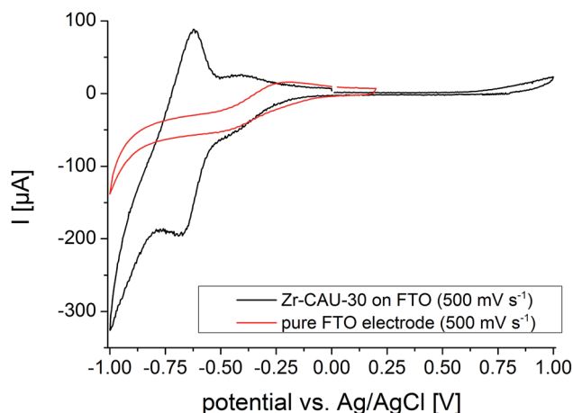
Fig. 12 CV curves of Zr-CAU-30 on FTO (black) and the pure FTO electrode (red) between -1 and 1 V and a scan rate of 500 \text{mV s}^{-1} .
