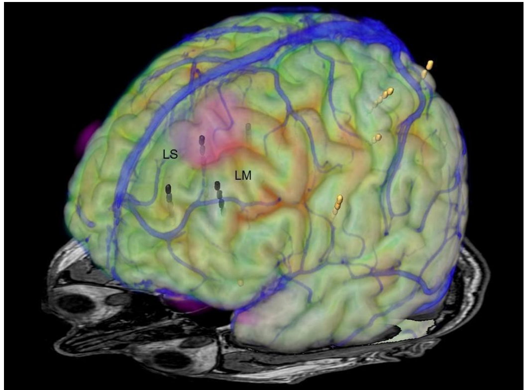
FIGURE 6: Image fusion of superficial veins, MRI, FDG-PET, DTI-MRI and depth electrodes
