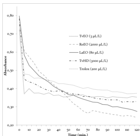
Figure 1. Reaction kinetics of three EOs, one HD and Trolox for 120 minutes. Abbreviations: EO: Essential oil; HD: Hydrosol; Tv: Thymus vulgaris ; Ro: Rosmarinus officinalis ; La: Lippia alba .
