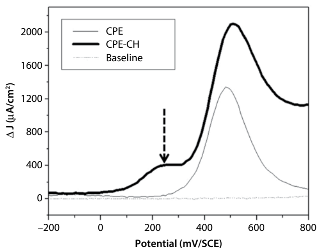
Figure 7 Square wave voltammograms of 75 \text{ mg L}^{-1} PCT at the bare CPE and CPE-CHr in PBS, with a pulse high of 90 mV, frequency of 400 Hz and scan increment of 15 mV.
