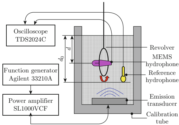
Fig. 10 The standing wave tube calibration device.
