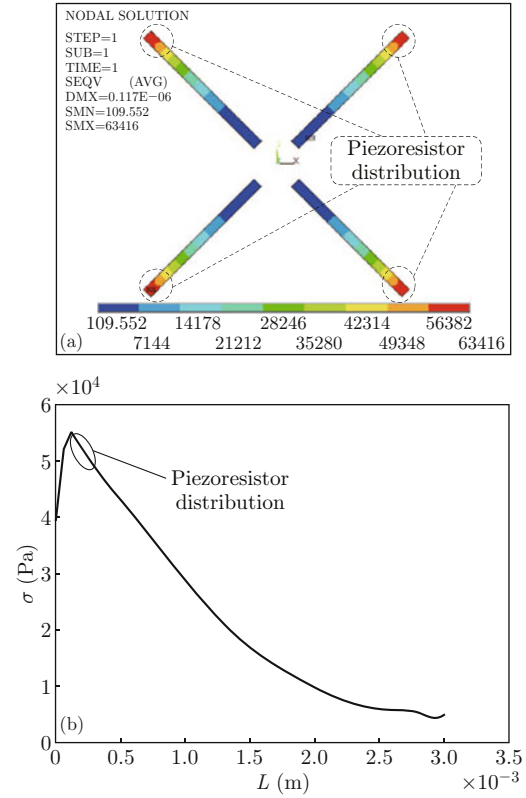
Fig. 5 (a) The stress-contour of cantilever beam; (b) Curve of cantilever stress distribution.
