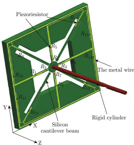
Fig. 2 Schematic of the bionic MEMS hydrophone.
