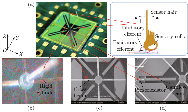
Fig. 8 Images of the hydrophone microstructure.
