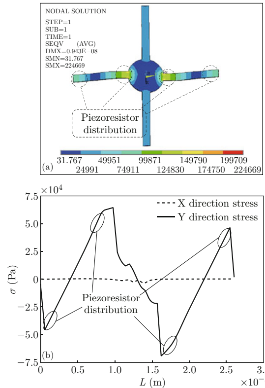
Fig. 6 (a) The stress-contour of cross-beam; (b) Curve of cross-beam stress distribution.
