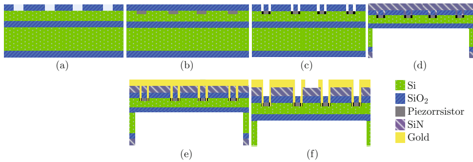
Fig. 7 The process of manufacturing technology. (a) Oxidation and ICP etching; (b) Implant boron to form piezoresistors and re-oxidation; (c) ICP etching and implantation dense boron; (d) PECVD epitaxy and ICP etching; (e) ICP etching and sputtering gold; (f) Gold etching and release the structure.
