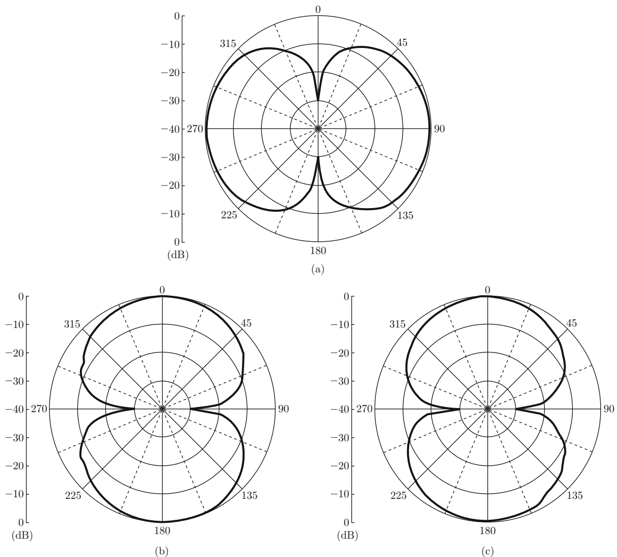
Fig. 12 (a) Directivity pattern of X direction; (b) Directivity pattern of Y direction; (c) Directivity pattern of Z direction.
