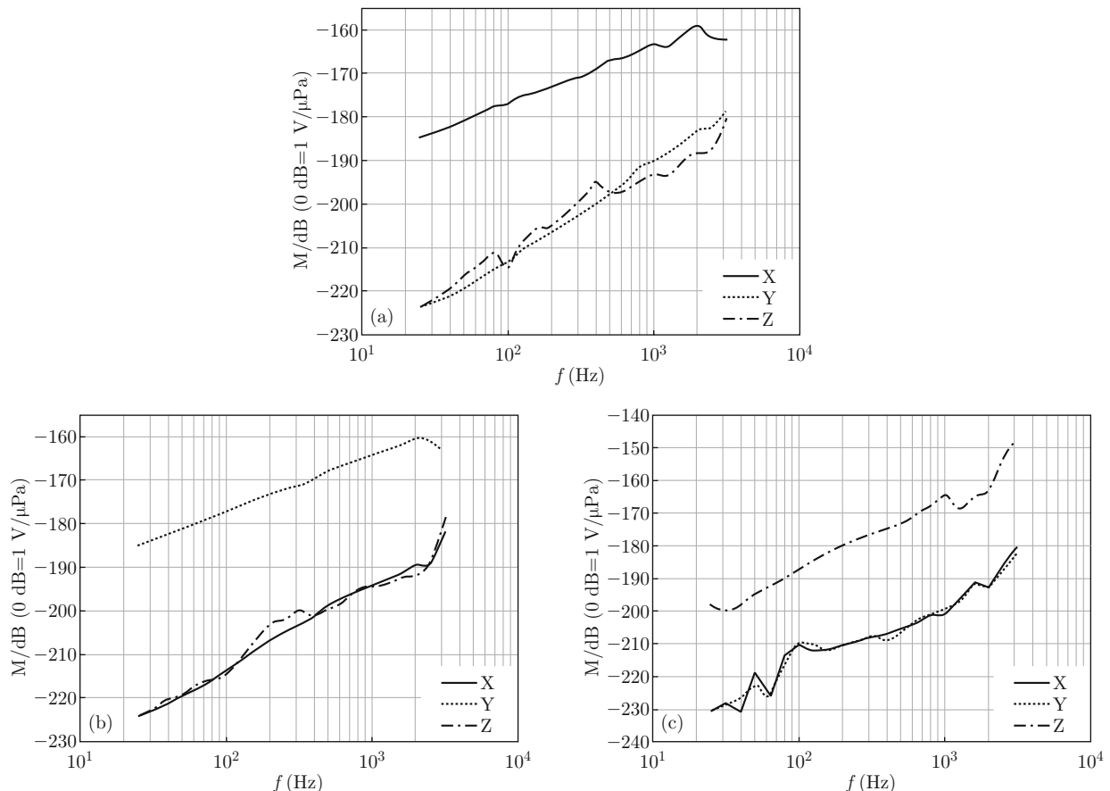
Fig. 11 (a) Frequency response curve of X direction (attenuation of 20 dB); (b) Frequency response curve of Y direction (attenuation of 20 dB); (c) Frequency response curve of Z direction (attenuation of 20 dB).
