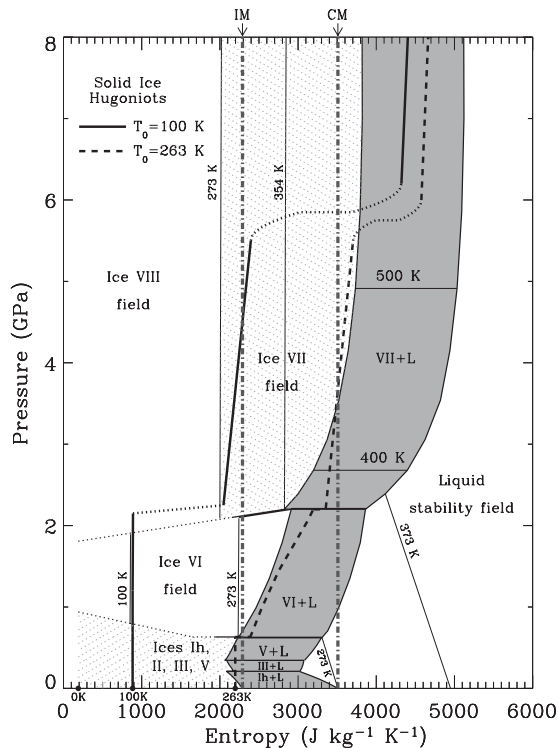
FIGURE 6. 100 and 263 K ice Hugoniots and partial simplified \text{H}_2\text{O} phase diagram in pressure-entropy space [3, 17-20]. IM and CM denote critical entropies for incipient and complete melting upon release to zero pressure. Both Hugoniots exit the ice VII-liquid boundary and enter the liquid field around 20 GPa (above plotted pressure range) [4]. Reproduced by permission of American Geophysical Union.
