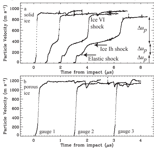
FIGURE 2. a. Particle velocity vs. time gauge records measured at 3-mm intervals within 100 K solid ice target subject to 1473 m s -1 impact by polycarbonate projectile producing 3-wave shock front and 2.1 GPa peak pressure [4]. Reproduced by permission of American Geophysical Union. b. Records from 1572 m s -1 impact to 1.4 GPa in 40 % porous ice at 150 K.
