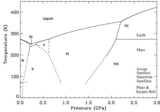
FIGURE 1. Partial H 2 O phase diagram showing only stable phases [3 and references within]. Mean surface temperatures of solar system objects noted on right.
