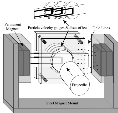
FIGURE 3. Sketch of particle-velocity gauge method for measuring Hugoniot states. U_S was determined from wave arrival time at each gauge. u_P was calculated from voltage signal, E , using Faraday's law, u_P = E/(LH) , gauge length L , and magnetic field strength H [4]. Reproduced by permission of American Geophysical Union.
