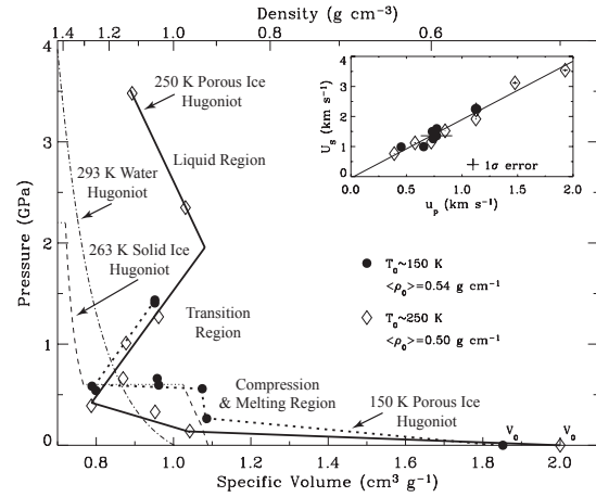
FIGURE 5. 40–45 % porous ice shock data compared to liquid water and solid ice Hugoniot. Data sources: \bullet this work, \diamond [13].
