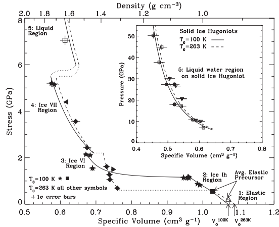
FIGURE 4. Solid ice Hugoniot centered at 100 K (solid) and 263 K (dashed) [4]. Dots connect the 5 Hugoniot regions. Data sources: \blacksquare \star this work, \blacktriangle \blacklozenge [7], \square [12], \nabla \odot [14], \blacktriangleright [15], \blacktriangleleft [16]. Reproduced by permission of American Geophysical Union.
