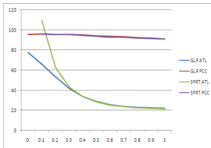
Figure 3: ATL and PCC for 5% nominal error rate, comparing GLR and SPRT
