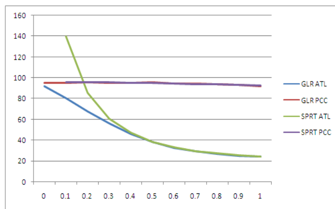
Figure 2: ATL and PCC for 1% nominal error rate, comparing GLR and SPRT
