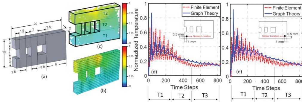
Figure 4. (a) The C-shaped part from Figure 3 is modified with two supports to provide a path for the heat in the overhang section to dissipate. (b) and (c) The heat flux during fusion of the last layer of the modified part with two supports specially designed estimated using the graph theoretic, and finite element-based approach respectively. (d) and (e), the heat flux trends observed at two locations on the part, in the left and right corner, respectively, corresponding to the three sections marked in (c).
