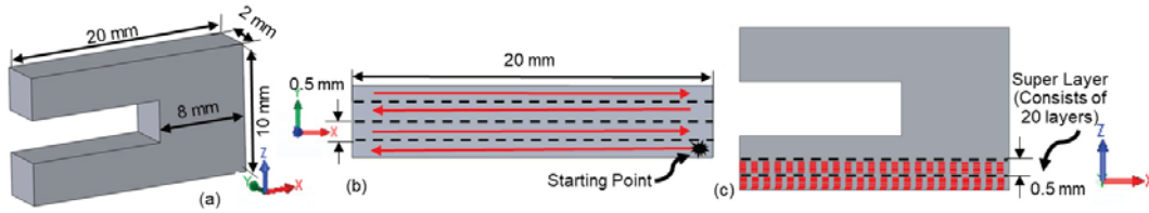
Figure 2. (a) Dimension of C-shape part in mm, (b) top view of C-shape part and scanning strategy in simulation, (c) side view of C-shape part.
