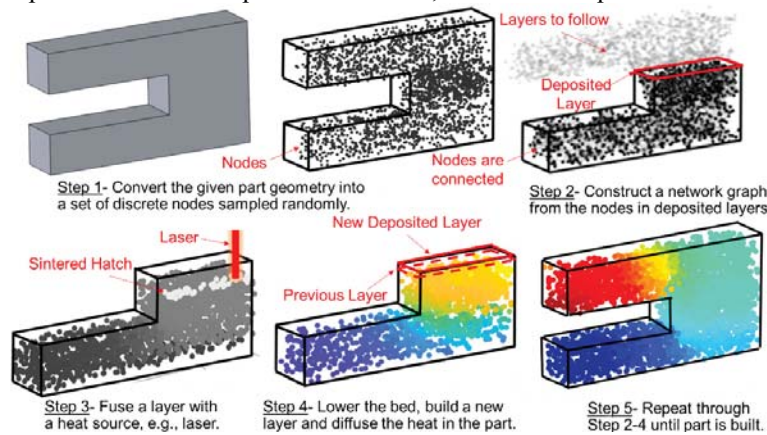
Figure 1. The five steps in the spectral graph theoretic approach used to estimate the heat flux in the part layer-by-layer. Here we show an embodiment of the laser powder bed fusion (LPBF) process.
