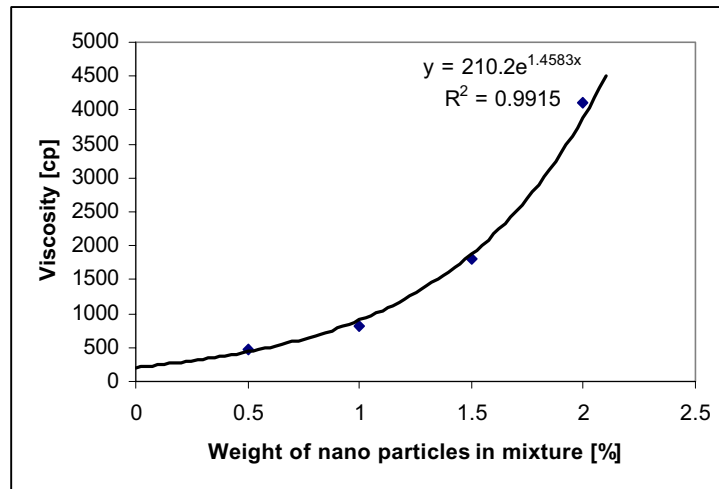
Fig. 10. Viscosity of photopolymer-nanoparticle mixture (measured at 1.0 rpm)
