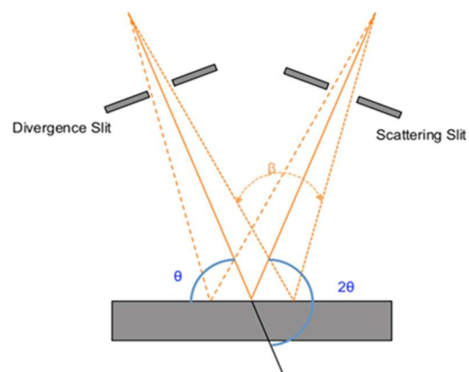
(a) Outline of the Thin film X-ray diffraction
