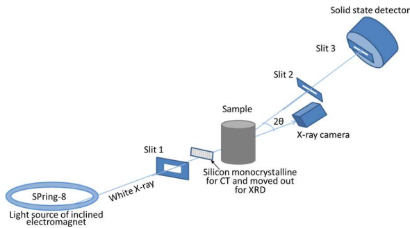
Fig.1. Schematic of the system for Non-destructive integrated CT-XRD method
