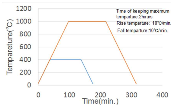
Fig. 4. Temperature program
