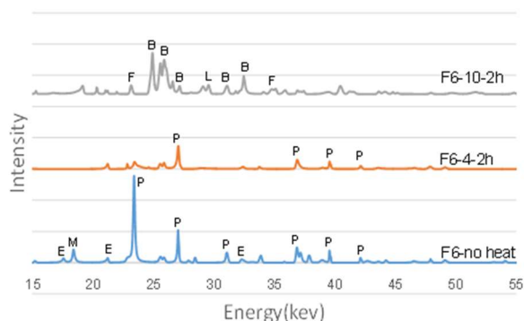
Fig. 6. The diffraction profile of F6 obtained by Thin film X-ray diffraction technique
