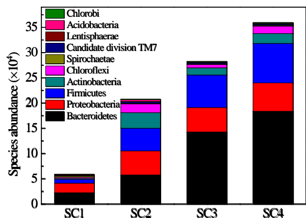
Fig. 6. Distribution of species number at the phylum level of sewage with different concentration
