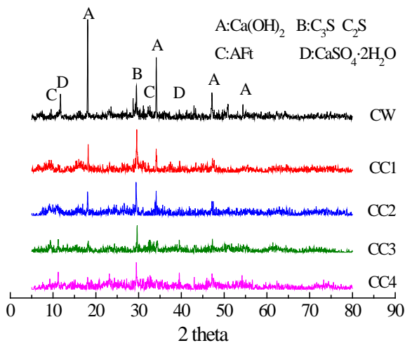
Fig. 13. XRD curves of the specimens in water and sewage
