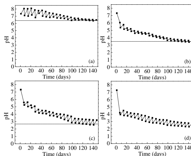
Fig. 3. Evolution diagrams of pH values of sewage with different concentration: a) SC1; b) SC2; c) SC3; d) SC4
