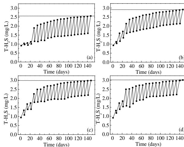
Fig. 4. Evolution diagrams of T-H 2 S values of sewage with different concentration: a) SC1; b) SC2; c) SC3; d) SC4
