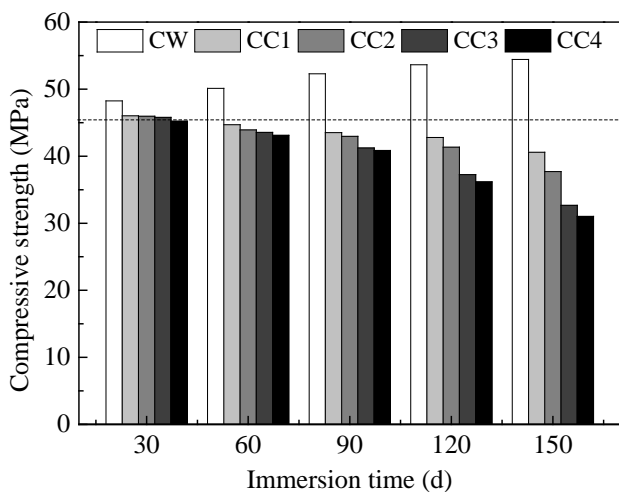
Fig. 11. Comparison of strength of concrete specimens in water and sewage
