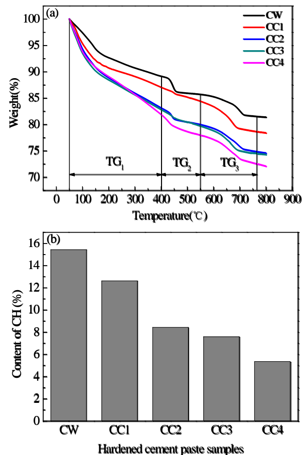
Fig. 14. Comparison of TGA of specimens in water and sewage: a) thermal-gravimetric curve; b) calcium hydroxide content
