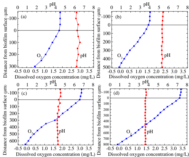
Fig. 8. Microelectrode test results of biofilms in sewage: a) BC1; b) BC2; c) BC3; d) BC4
