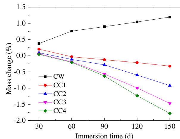
Fig. 10. Comparison of mass change of concrete specimens in water and sewage
