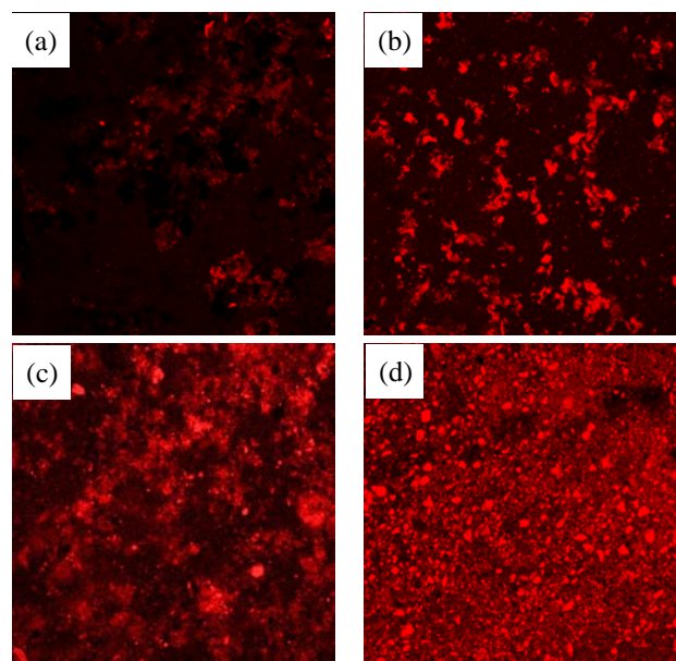
Fig. 7. CLSM images of biofilms in sewage: a) BC1; b) BC2; c) BC3; d) BC4
