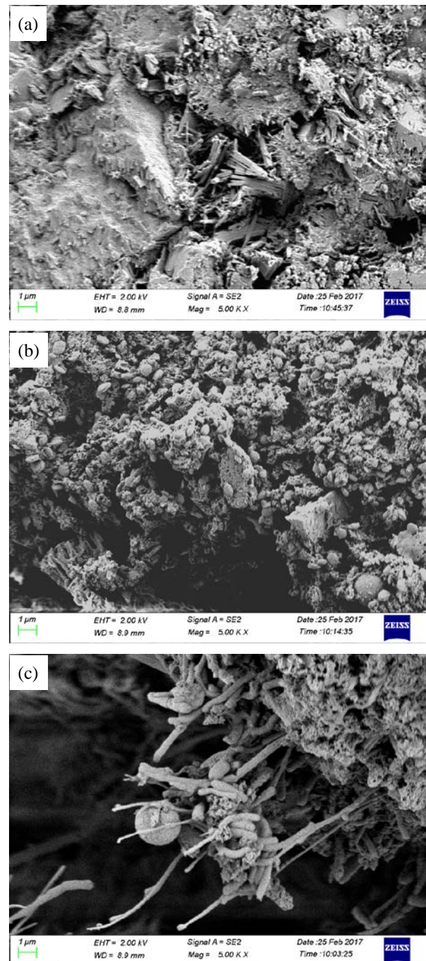
Fig. 12. SEM micrographs of concrete specimens in sewage: a) CW; b) CC2; c) CC4
