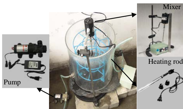
Fig. 1. In-house simulation chamber for sewage corrosion test
