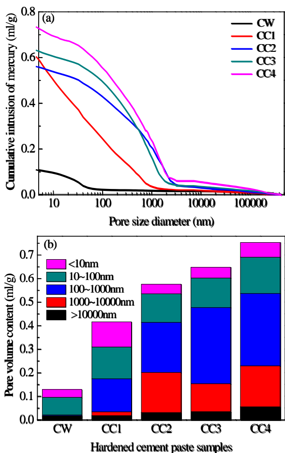
Fig. 15. Comparison of pore structure of specimens in water and sewage: a) cumulative mercury quantity curve; b) pore size distribution column
