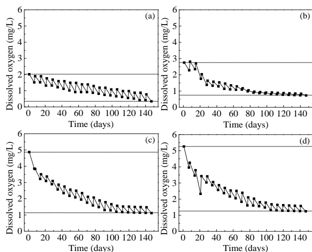
Fig. 5. Evolution diagrams of O 2 values of sewage with different concentration: a) SC1; b) SC2; c) SC3; d) SC4
