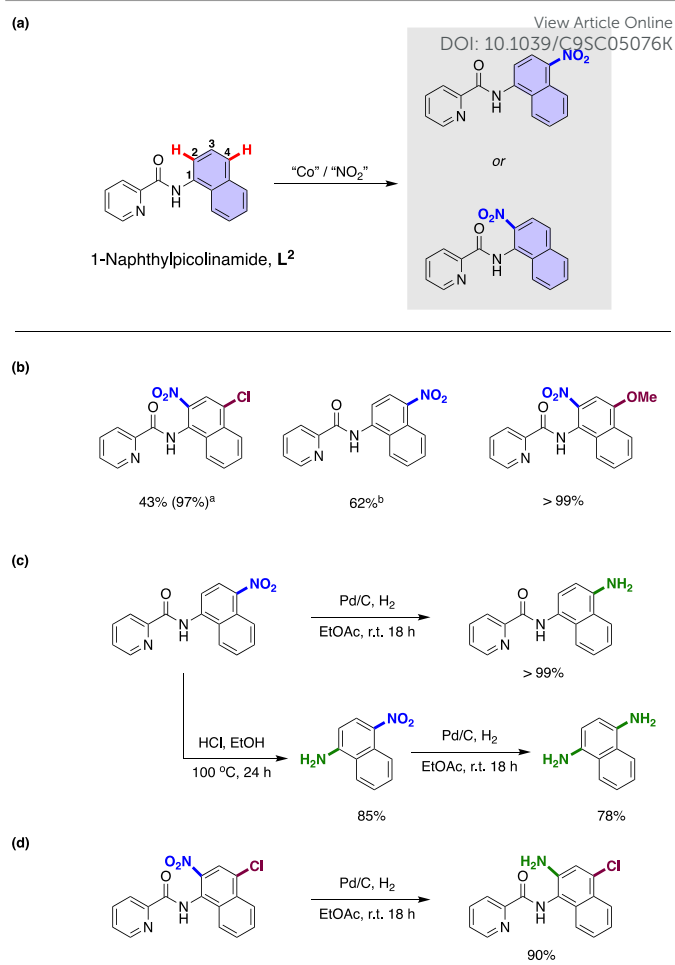
Scheme 3: (a) 1-Naphthylpicolinamide substrates used in the experimental work; nitration at either the 2- or 4-position for the 1-naphthylpicolinamide. (b) Products isolated from the Co-catalysed remote nitration of 1-naphthylpicolinamide substrates; Reaction conditions: 0.50 mmol 1-naphthylpicolinamide substrate, 20 mol% Co(NO 3 ) 2 ·6H 2 O, 4.0 equivalents TBN, 3.5 mL AcOH, r.t., 18 h. a 6.0 equivalents of TBN. b Only the 4-substituted product could be successfully isolated, and the yield shown is of this regioisomer. (c) Examples of product upgrading of the nitrated compound obtained from 1-naphthylpicolinamide. (d) Examples of product upgrading of the nitrated compound obtained from 4-chloro-substituted 1-naphthylpicolinamide substrate.
