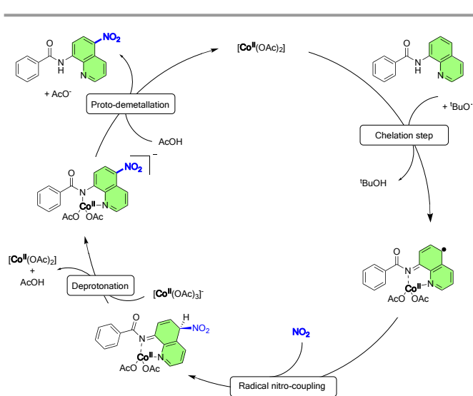
Scheme 2: Proposed mechanism for the remote nitration of 8-aminoquinolinamide substrates catalysed by \text{Co}(\text{OAc})_2 at the 5-position based on the computational studies in from this work. Note: the \text{NO}_2 is formed in-situ from the decomposition of TBN (see Equations 1 and 2).
