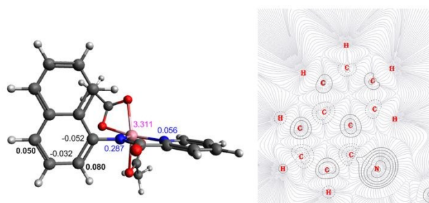
Figure 4: Left: Molecular structure with calculated spin densities for 5 Int 1-L 2 obtained using DLPNO-CCSD/def2-tzvp highlighting the spin accumulated at the 2- and 4-positions on the 1-aminonaphthyl moiety. Right: QTAIM wavefunction analysis of spin density gradients, focusing on the 1-aminonaphthyl moiety.
