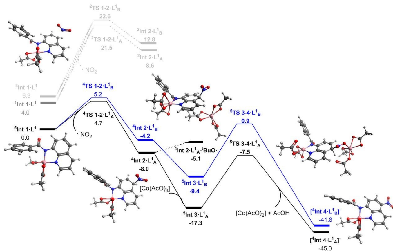
Figure 2: Solvated free energy surface ( \Delta G_{298} ) for the nitration of 8-aminoquinolinamide calculated with DLPNO-CCSD(T)/def2-TZVP. Black (A) and blue (B) lines represent high spin nitration at the 5 and 7 positions respectively. Dark grey represents first excited state optimised geometry of Int 1-L 1 . Light grey represents the corresponding low spin pathway. Calculated geometries shown are for the observed 5-position nitration via the high spin mechanism.
