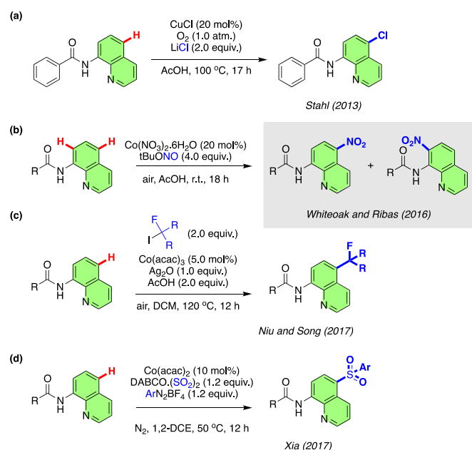
Scheme 1: (a) Cu-catalysed remote chlorination reported by Stahl. (b) First Co-catalysed remote nitration reported by Whiteoak and Ribas. (c) Co-catalysed remote perfluoroalkylation reported by Niu and Song. (d) Co-catalysed remote sulfonylation reported by Xia.
