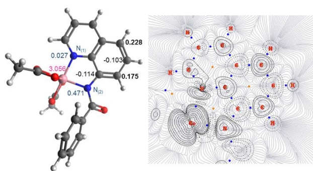
Figure 1: Left: Molecular structure with calculated spin densities for 5 Int 1-L 1 obtained using DLPNO-CCSD/def2-tzvp highlighting the spin accumulated at the 5- and 7- positions on the 8-aminoquinolinamide ligand. Right: QTAIM wavefunction analysis of spin density gradients and bond critical points, focusing on the 8-aminoquinoline moiety.
