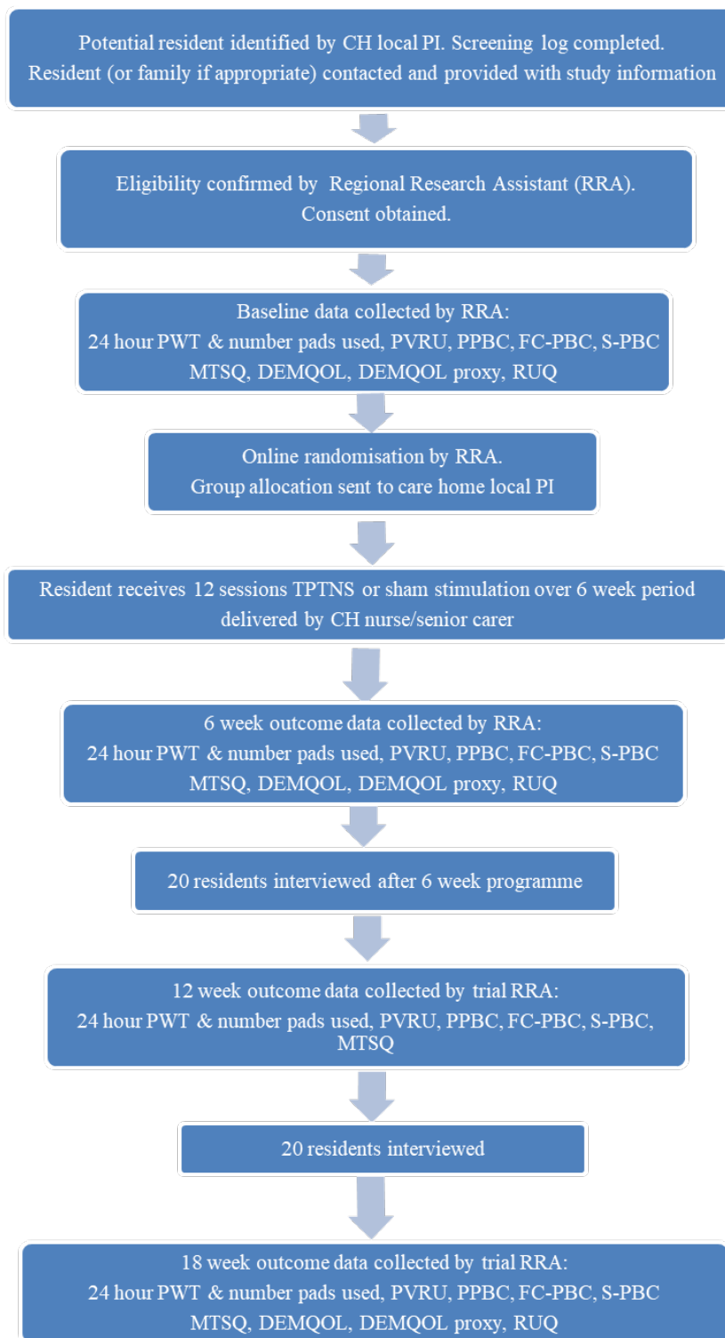
Figure 1: Resident Flowchart
