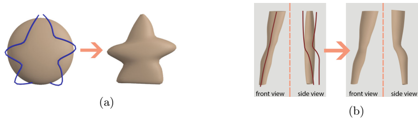
Fig. 3: ODE-driven Sketch-based deformations: (a)the deformation process of an organic shape represented by an ellipsoid and its 2D silhouette contour, and the deformed shape of the ellipsoid, (b) a leg that has been deformed by single-view sketch strokes before, now get further deformed in accordance with free form red-colored curves
