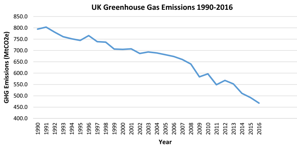
Fig. 2 GHG emissions national statistics 1990–2016 (BEIS 2018b)
