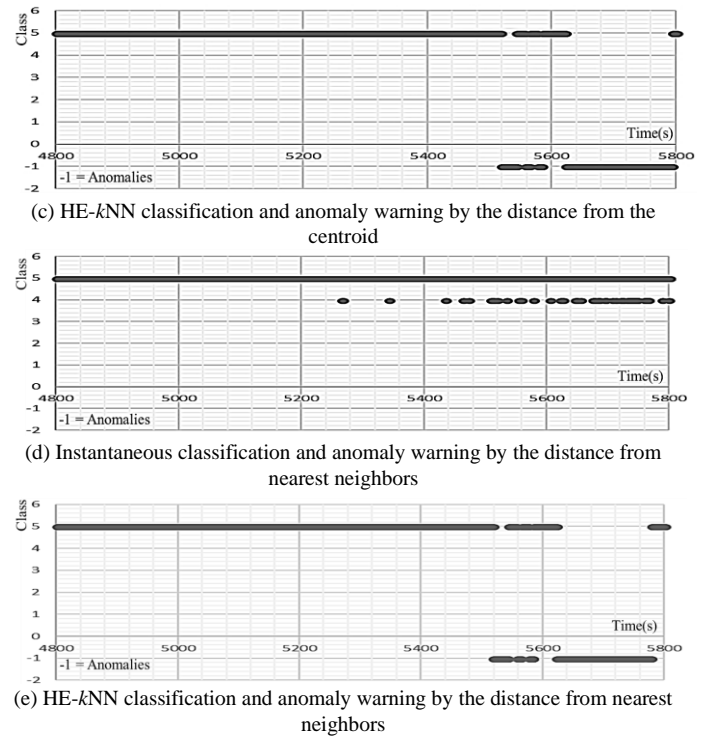
Fig. 9. Waveforms and results from the ELV dc air conditioner on malfunction in fan
