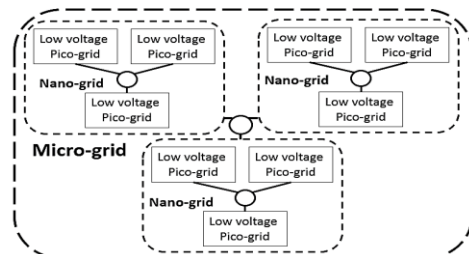
Fig. 1. ELV dc pico-grids forming into a micro-grid
