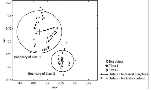
Fig. 6. Anomaly warning criteria in HE-kNN
