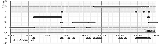
(b) Instantaneous classification and anomaly warning by the distance from the centroid
