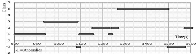
(e) HE-kNN classification and anomaly warning by the distance from nearest neighbors
