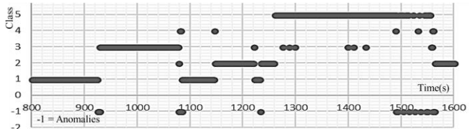
(d) Instantaneous classification and anomaly warning by the distance from nearest neighbors
