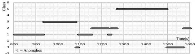
(c) HE-kNN classification and anomaly warning by the distance from the centroid
