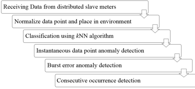
Fig. 5. Hierarchy processes in HE-kNN technique
