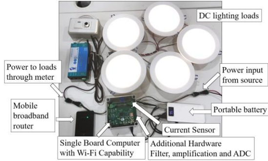
Fig. 3. An example of the slave meter in an ELV dc pico-grid of lightings
