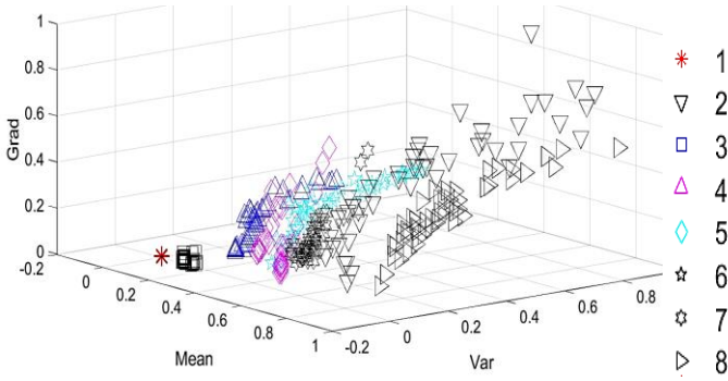
Fig. 10. Clusters for the ELV 3 loads dc grid
