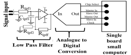
Fig. 4. Hardware system diagram of the slave meter
