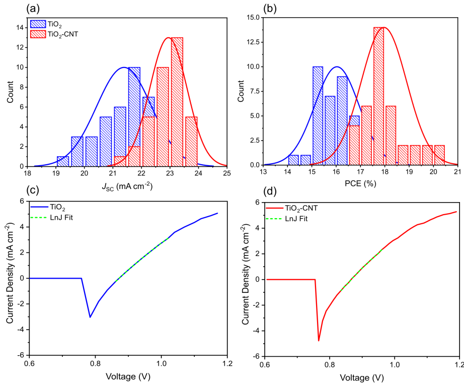
Figure 2. Histograms of photovoltaic parameters J_{\text{sc}} (a) and PCE (b) for TiO 2 and TiO 2 -CNT PSCs. Semi-log plots of the dark J-V measurements for TiO 2 (c) and TiO 2 -CNT (d) PSCs.
