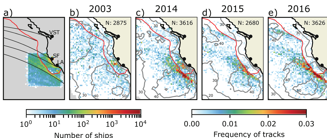
Figure 1. Interannual variation in shiptrack locations. (a) Locations of ships determined using AIS data at the satellite overpass time in 2015. Thin black lines show major shipping routes, and the orange dots the locations of the ports of Vancouver/Seattle, San Francisco/Oakland, and Los Angeles/Long Beach. (b–e) Frequency of occurrence of identified shiptracks for the years 2003, 2014, 2015, and 2016. The red line is the U.S. Pacific ECA. Thin gray lines show the percentage annual average liquid cloud fraction from MODIS. The number of identified tracks each year is in the upper right of each subplot. Land and locations viewed by fewer than 100 granules are masked.
