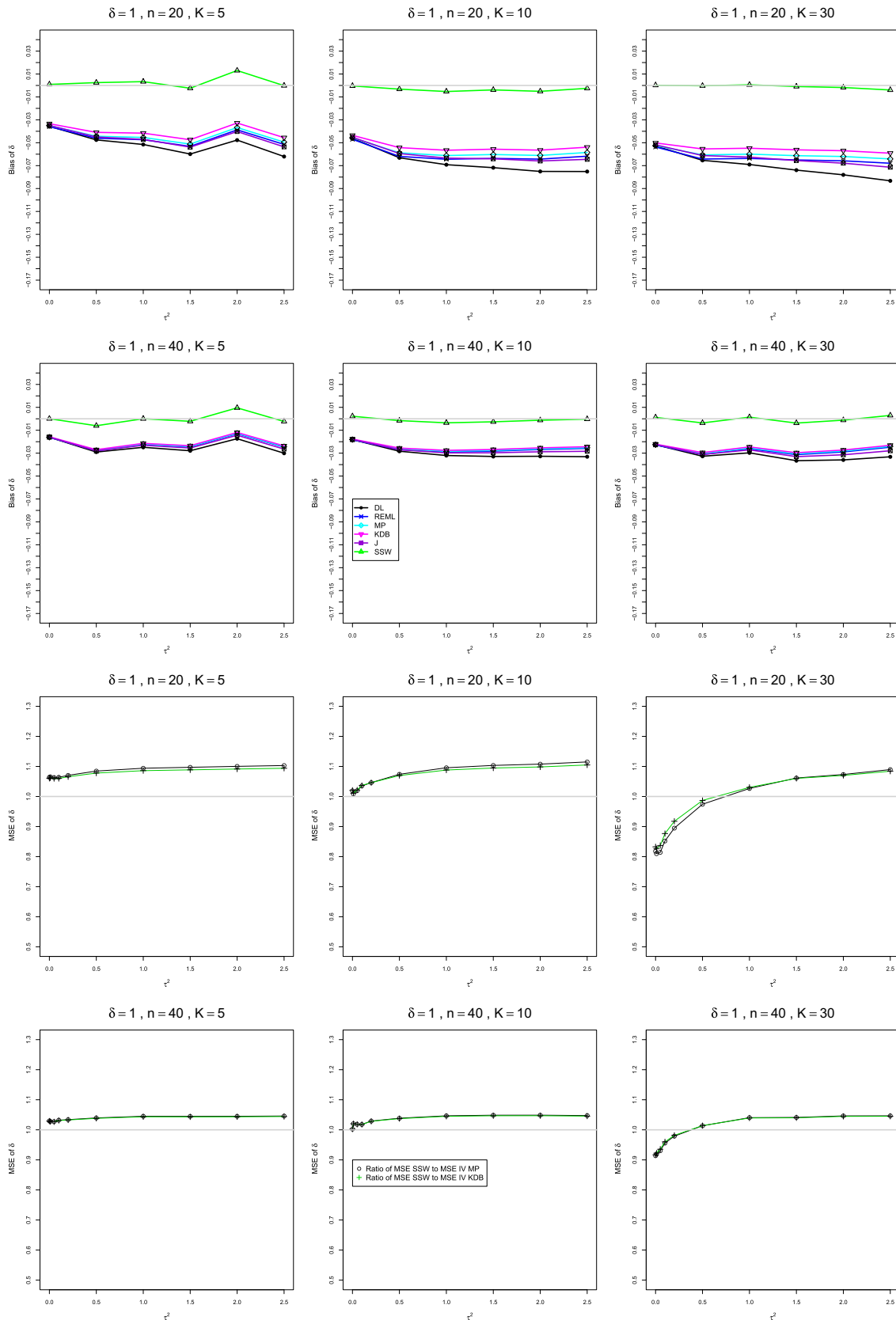
FIGURE 5 Standardized mean difference: Bias of the estimators of \delta and ratio of mean squared errors (MSEs) of SSW to inverse-variance-weighted estimators when \delta = 1 , q = .5 , n = 20, 40 , and K = 5, 10, 30 . Light gray line at 0 for bias and at 1 for the ratio of MSEs. DL, DerSimonian-Laird; KDB, Kulinskaya-Dollinger-Bjørkestøl; J, Jackson; MP, Mandel-Paule; REML, restricted maximum-likelihood [Colour figure can be viewed at wileyonlinelibrary.com ]
