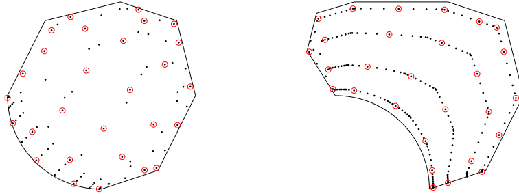
Figure 4: Convex and concave edge polygonal elements of Figures 1-2 with basic cubature nodes by splitting and arc blending (91 and 223 small dots, respectively), and compressed Caratheodory-Tchakaloff nodes (28 small circles), for ADE = 6 .
