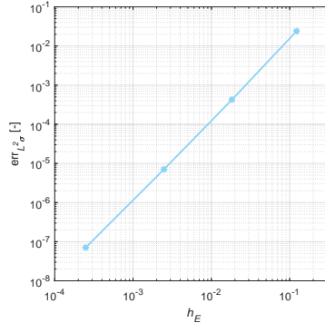
Figure 6: Infinite plate with hole. L^2 error norm for the Cauchy stress vs mesh size h_E for k = 2 VEM approximation.
