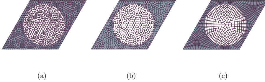
Figure 7: Asymptotic homogenization. Parallelogram unit cell with circular inclusion ( v_f = 0.5 .) Representative mesh types. (a) Tri-mesh. (b) Voro-mesh. (c) Quad-mesh
