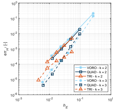
Figure 8: Asymptotic homogenization. H^1 error norm vs mesh size h_E for k = 2 and k = 3 VEM approximations of the homogenization problem.
