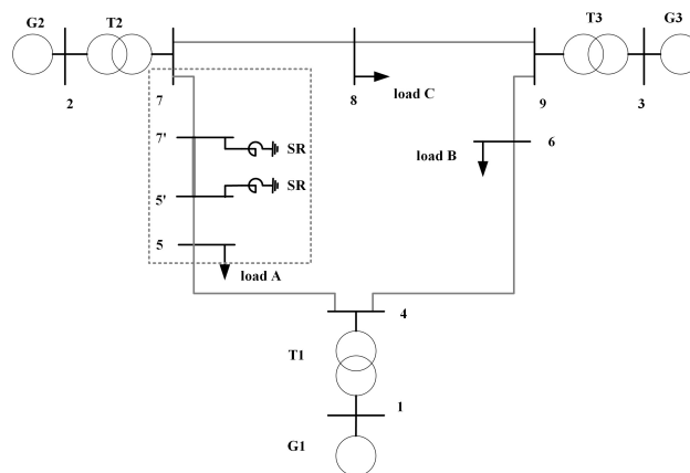
Figure 3. Single line diagram of a WSCC 3-machine 9-bus test system with a mixed line: a cable of 40 km is inserted in line 7-5, with two shunt reactors of 2 \times 100 MVAR ratings to compensate the reactive power requested by the cable.
