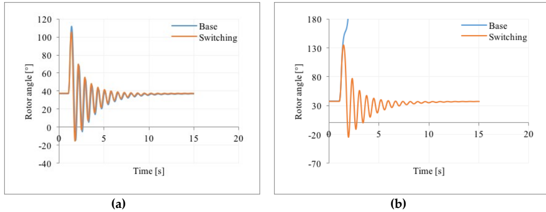
Figure 12. Rotor angle of the synchronous machine of Area 1 for a three-phase fault on Area 1 side: (a) Time results for clearing fault time t_{\text{clear}} = 170 ms; (b) Time results for clearing fault time t_{\text{clear}} = 201 ms (critical clearing time t_{\text{CCT}} ).
