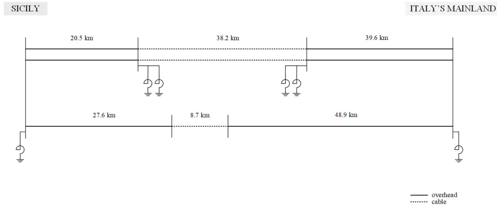
Figure 7. Single line diagram of existing 400 kV interconnections between Sicily and Italy's mainland. Overhead sections are indicated with continuous lines; cable sections are indicated with dashed lines.
