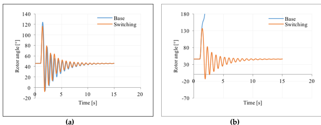
Figure 10. Rotor angle of the synchronous machine of Area 1 for a three-phase fault on Area 1 side: (a) Time results for clearing fault time t_{clear} = 170 ms; (b) Time results for clearing fault time t_{clear} = 191 ms (critical clearing time t_{CCT} ).
