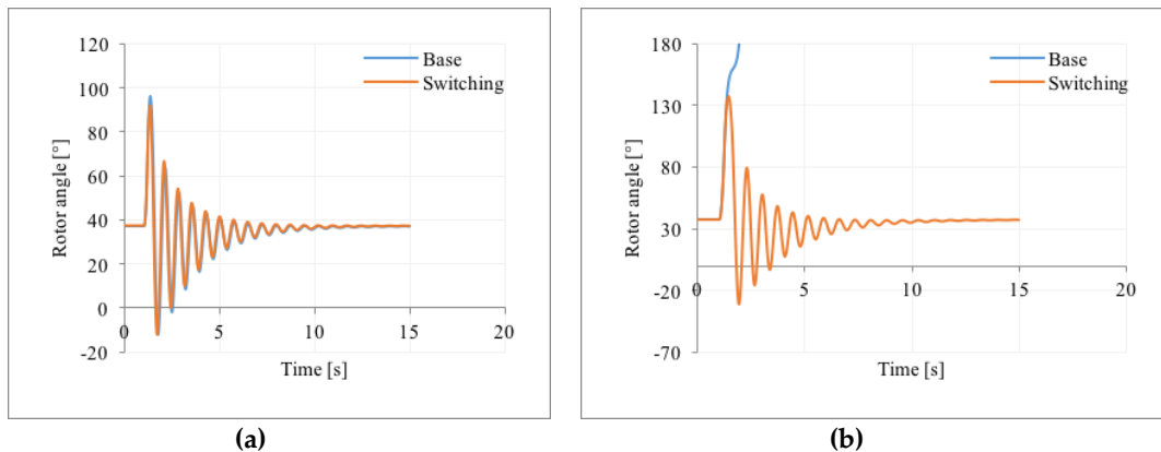
Figure 13. Rotor angle of the synchronous machine of Area 1 for a three-phase fault on Area 2 side: (a) Time results for clearing fault time t_{\text{clear}} = 170 ms; (b) Time results for clearing fault time t_{\text{clear}} = 230 ms (critical clearing time t_{\text{CCT}} ).
