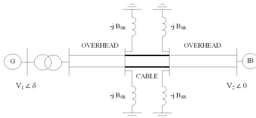
Figure 1. Simple test system: one synchronous machine is connected to infinite bus through a double-circuit mixed overhead-cable line. The mixed line is compensated with four shunt reactors of 220 MVAR each, installed at the cable ends.
