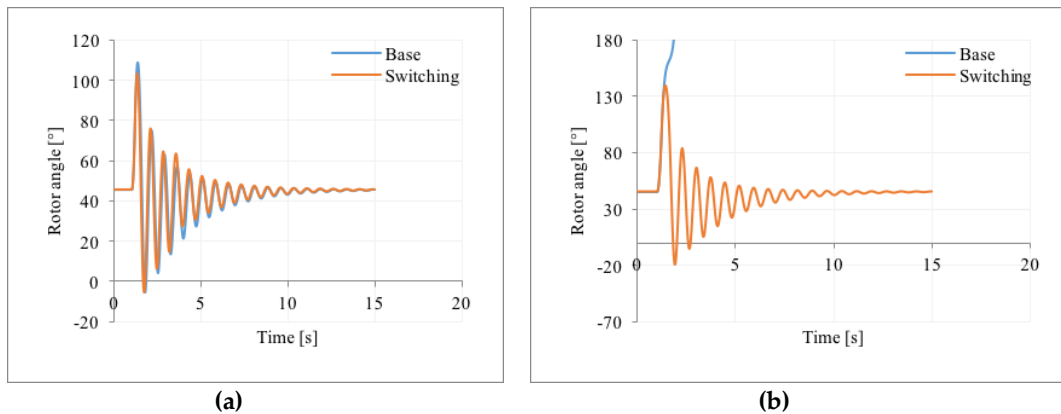
Figure 11. Rotor angle of the synchronous machine of Area 1 for a three-phase fault on Area 2 side: (a) Time results for clearing fault time t_{\text{clear}} = 170 ms; (b) Time results for clearing fault time t_{\text{clear}} = 215 ms (critical clearing time t_{\text{CCT}} ).
