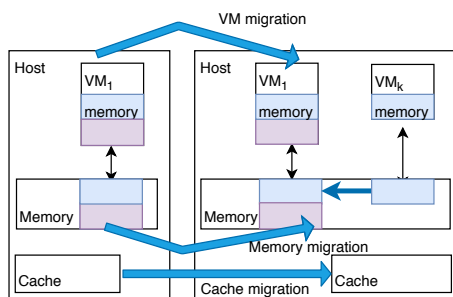
FIGURE 25. General scheme of the VM migration.
