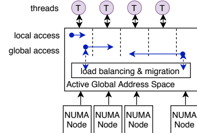
FIGURE 10. General scheme of the active global address space.
