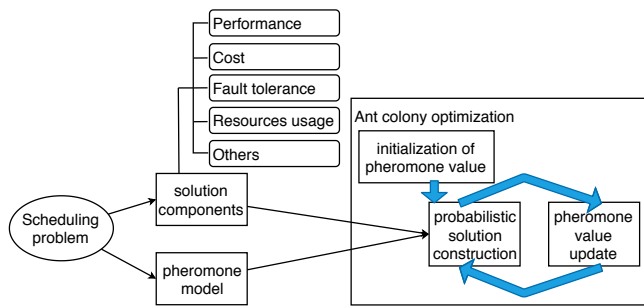
FIGURE 16. Ant colony optimisation in scheduling.
