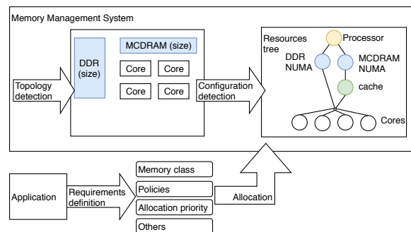
FIGURE 4. Overview of the memory locality in HPC.
