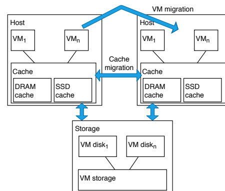
FIGURE 22. General scheme of the cache organisation in Cloud.
