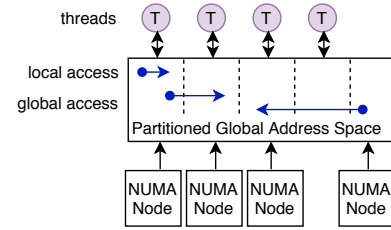
FIGURE 9. General scheme of the partitioned global address space.
