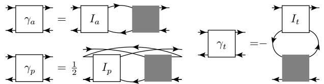
FIG. 4. Bethe-Salpeter equations in the three two-particle channels, relating the reducible ( \gamma_r ) and irreducible ( I_r ) vertices self-consistently in the parquet formalism.
