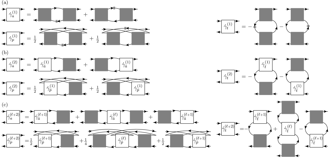
FIG. 5. Multiloop flow equations for the four-point vertex in a general fermionic model. (a) Standard truncated, one-loop flow, where a line with double dashes denotes \partial_\Lambda G . (b) Two-loop correction (upon inserting the one-loop contributions, one obtains two loops connecting full vertices). (c) Higher-loop corrections starting from \ell+2=3 , which contain the additional contribution (center part) where vertices from the complementary channels are connected by two bubbles.
