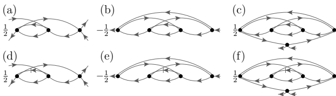
FIG. 6. (a-c) Some diagrams that are included in the parquet approximation and only partially contained in one-loop fRG. (d-f) One particular differentiated diagram for each of the diagrams (a-c) [the (gray, thin) line with a dash stands for \partial_\Lambda G^0 ] that is not part of the standard truncated flow, but included in mfRG.
