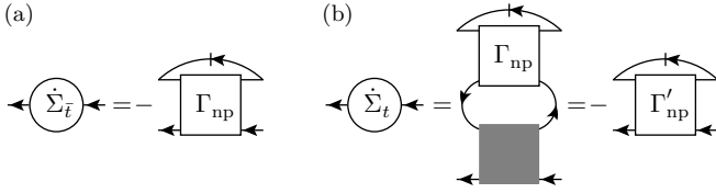
FIG. 9. Rewriting of the corrections to the self-energy flow: (a) \dot{\Sigma}_{\bar{t}} can be expressed by a nonparquet vertex \Gamma_{np} contracted with the single-scale propagator S . (b) \dot{\Sigma}_t , obtained by connecting \dot{\Sigma}_{\bar{t}} and \Gamma by a t bubble, then involves a bubble connecting a nonparquet and parquet vertex, which yields another nonparquet vertex \Gamma'_{np} , contracted with S .
