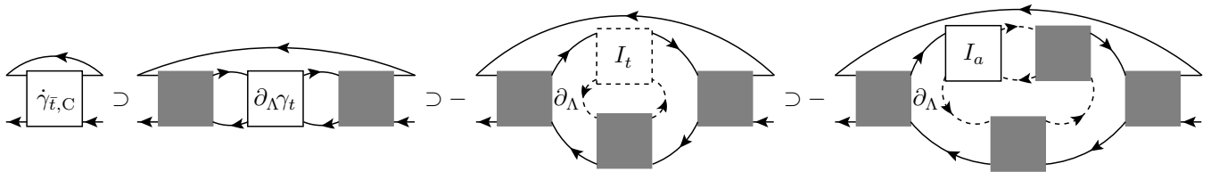
FIG. 8. Special diagrams contributing to \dot{\Sigma}_{\bar{i}} . In the last two diagrams, we consider a scenario where the differentiated line is contained in one of the dashed contributions.
