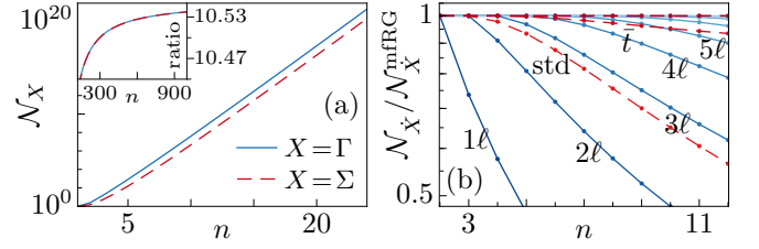
FIG. 10. Logarithmic plots for the number of diagrams at interaction order n for both vertex and self-energy. (a) \mathcal{N}_\Gamma, \mathcal{N}_\Sigma grow exponentially for large n (inset: the ratio of subsequent elements approaches a constant). (b) The cumulative low-loop vertex flows ( 1\ell up to 5\ell ) and the self-energy flows \tilde{\Sigma}_{\text{std}} (labeled std) and \tilde{\Sigma}_{\text{std}} + \tilde{\Sigma}_{\tilde{t}} (labeled \tilde{t} ) miss differentiated parquet diagrams. However, the full multiloop flow for vertex and self-energy generates all differentiated parquet diagrams to arbitrary order in the interaction.
