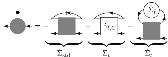
FIG. 7. Multiloop flow equation for the self-energy, adding two corrections ( \dot{\Sigma}_{\bar{t}} , \dot{\Sigma}_t ) to the standard fRG flow, \dot{\Sigma}_{\text{std}} . The (black, thick) line with a dash denotes the single-scale propagator S .
