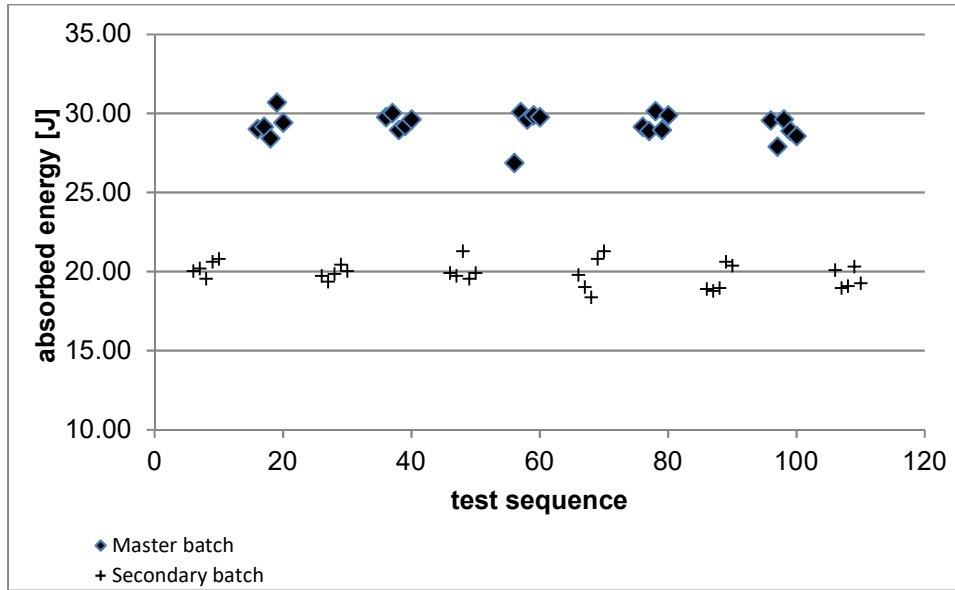
Figure 3: Absorbed energy values of 30 test pieces of ERM-FA013by, compared with 25 test pieces of ERM-FA013ba; data are displayed in the actual test sequence.
