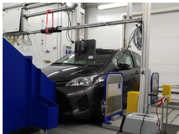
Figure 45: Vehicle TA008
