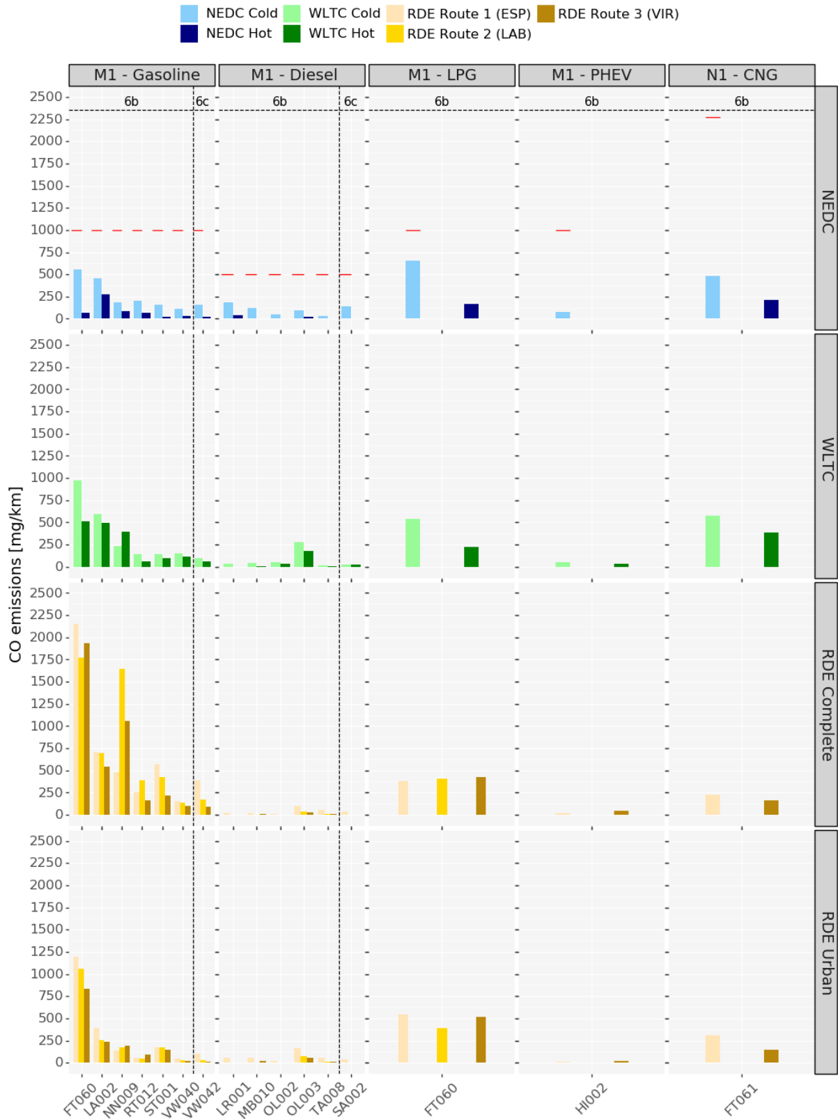
Figure 5: CO emissions for Euro 6b and Euro 6c vehicles over the NEDC laboratory cold and hot tests (top panel), the WLTC laboratory cold and hot tests (second panel) and on-road tests (third panel for complete trip and bottom panel for urban section). On the top panel, horizontal red lines stand for the CO limit applicable on the Cold NEDC.
