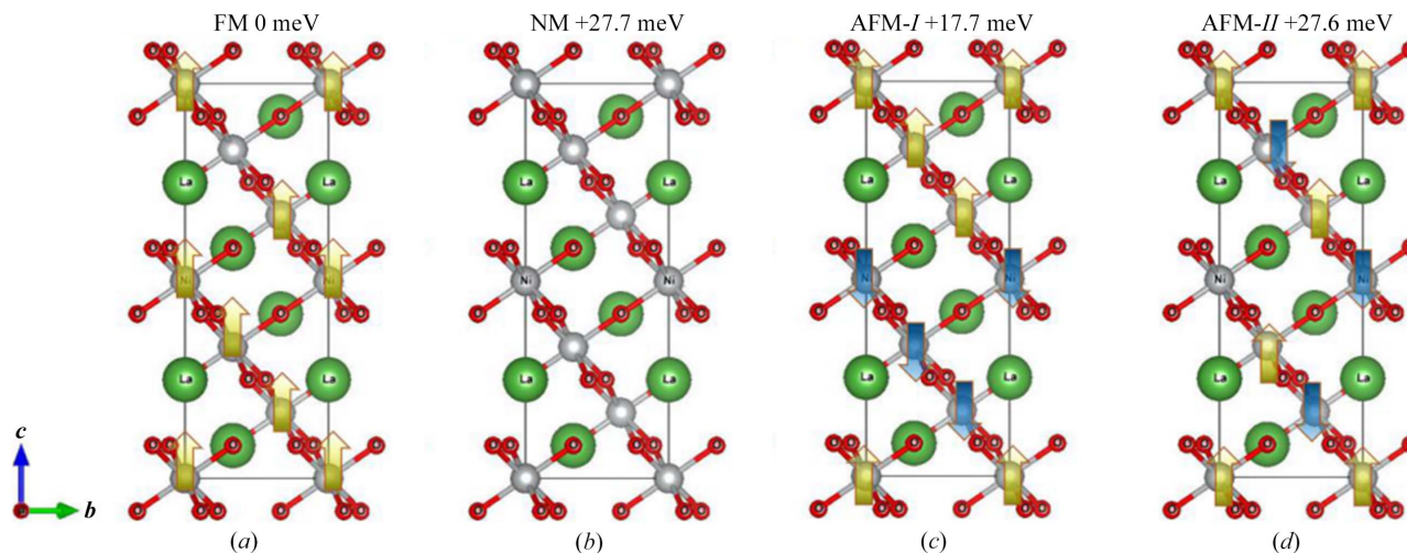
Figure 1 Crystal structures of LaNiO 3 ; the different magnetic structures including (a) FM, (b) NM, (c) AFM-I and (d) AFM-II are taken into consideration.
