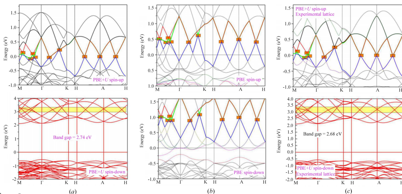
Figure 2 Calculated band structures of \text{LaNiO}_3 using (a) GGA+ U and (b) GGA methods at its optimized equilibrium lattice constants. For (c), the experimental lattice constants are selected during the electronic structure calculations.
