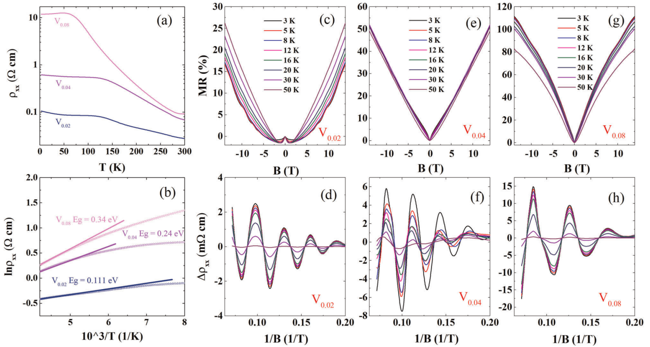
Fig. 2 Temperature dependence of the resistivity and the magnetoresistance (MR) of V:BSSTS. a The temperature dependence of the resistivity for crystals with different V contents. b Natural logarithm of the resistivity plotted against inverse temperature for different doping levels, linearly fitted to determine the band gaps. c, e, g The magnetoresistance at 3 – 50 K with different V-doping levels. d, f, h SdH oscillation patterns obtained from the MR curves and plotted as a function of 1/B
