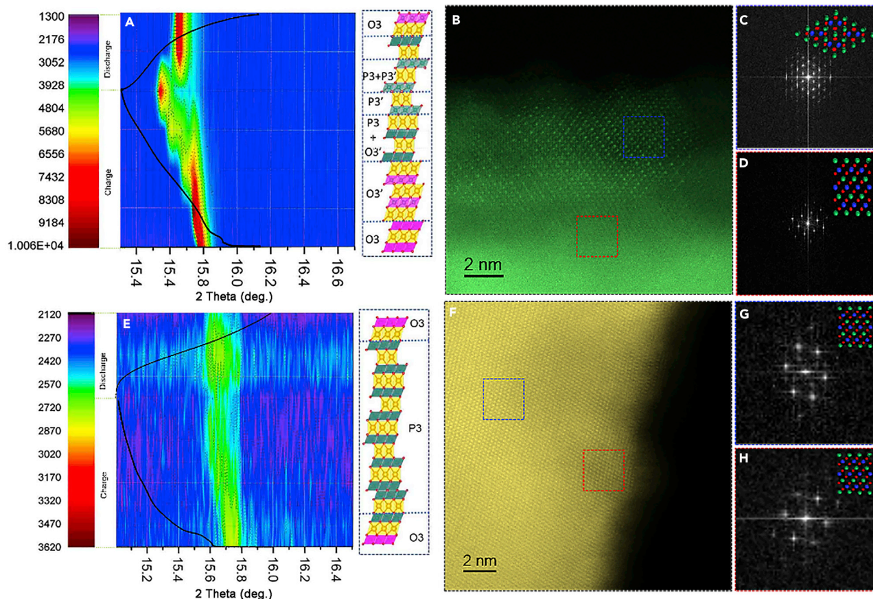
Figure 4. The Structure Evolution of P-NMNM and C-NMNM after Long-Term Cycle
