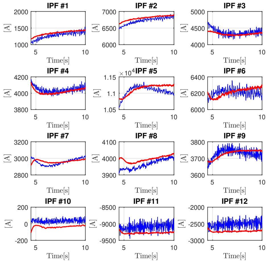
Figure 50: Simulated and experimental PFC currents for pulse #74104, obtained with the existing EAST controller. The experimental signal is shown in blue, while the simulated one is in red.
