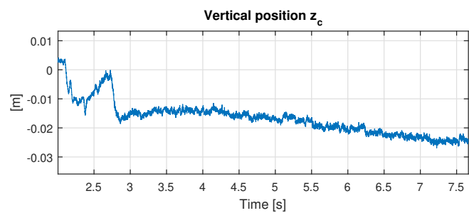
Figure 67: Plasma centroid vertical position for EAST pulse #77472.
