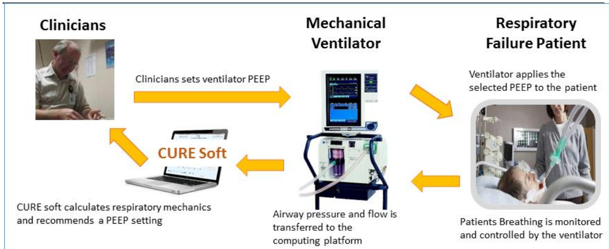
Figure 2: CURE software application for respiratory mechanics monitoring in the ICU [11].
