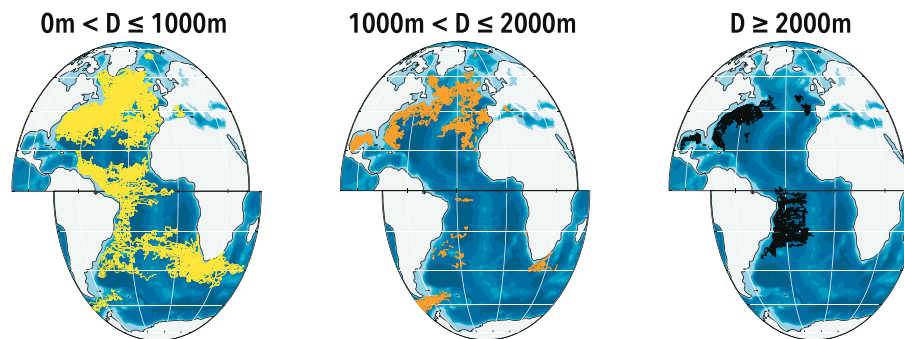
Figure 12. Subsurface float trajectories binned by depth, from left to right: 0–1,000 m; 1,000–2,000m; and 2,000m and deeper. Data source is the AOML PhOD subsurface drifter database, which currently houses all subsurface data collected through end of 2015 (Ramsey et al., 2018; https://www.aoml.noaa.gov/phod/float_traj/ ).
