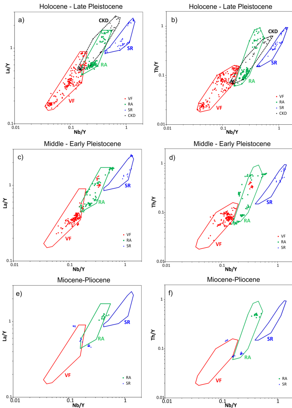
5 Figure 8 Discrimination diagrams for different volcanic zones in Kamchatka. The fields are drawn based on Holocene-late Pleistocene compositions. Coloured symbols show compositions of glasses according to their estimated ages and present-day location: Holocene-late Pleistocene (a, b), middle –early Pleistocene (c-d), and Miocene-Pliocene (e-f).
