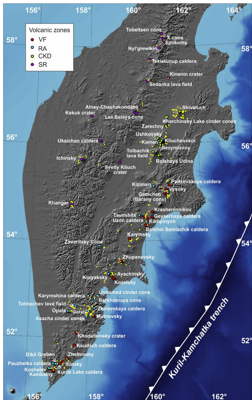
5 Figure 1 Volcanoes and samples presented in TephraKam. Large red circles with labels – volcanic centers; yellow circles – sample locations. Note that Kamchatka hosts more presently inactive volcanic centers than shown on the map, but tephra samples from these extinct volcanoes were not available for this study. The background image is drawn by the authors using public domain datasets SRTM for landmass (Farr et al., 2007) and GEBCO for ocean floor (Smith, Sandwell, 1997).
