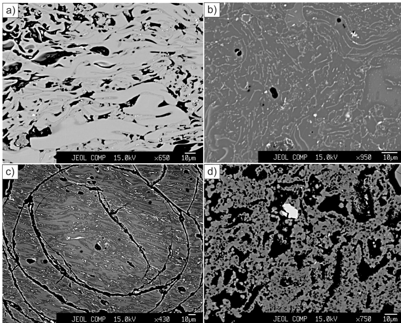
5 Figure 6 Back-scattered electron images of glass devitrification in welded tuffs: a) Slight alteration along welded glass particles (Sample 198-75, Karymsky/Stena-Sobolinaya caldera); b) More advanced alteration, precipitation of magnetite (sample 169-75, Karymsky/Stena-Sobolinaya caldera); c) Strong devitrification, developed perlite texture (sample 1989L-97b, unknown source/Alney-Chashakondzha?); d) Complete devitrification (sample PAU-8; Puzhetka caldera, no glass preserved).
