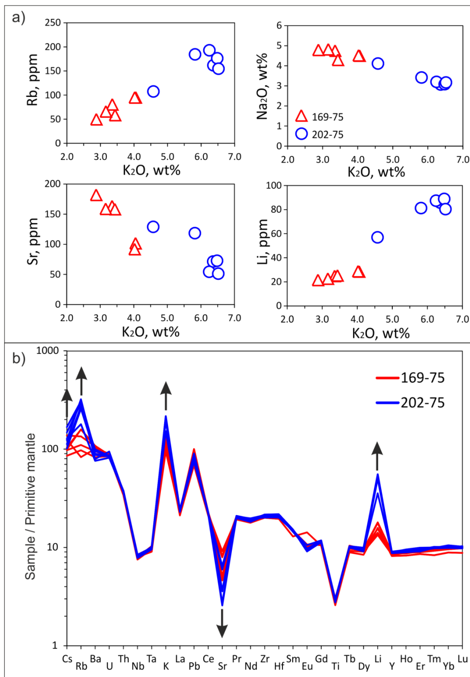
5 Figure 7 Illustration of chemical effects of secondary alteration on major and trace element composition of glass from welded tuffs: a) Covariations of mobile elements; b) Trace elements normalized to primitive mantle composition (McDonough and Sun, 1995). Arrows denote effect of alteration. Samples 169-75 (less altered) and 202-75 (more altered) are from Stena-Sobolinaya caldera and likely belong to the same unit judging from very close concentrations of immobile elements.
