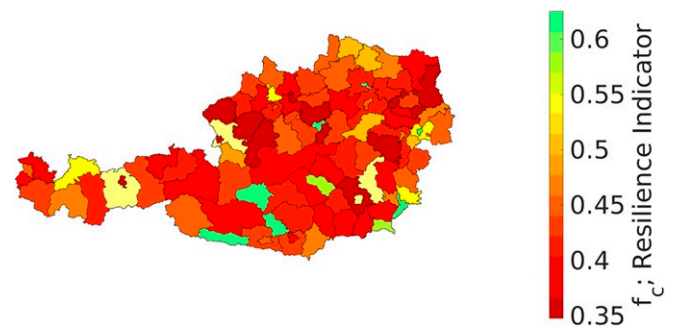
Fig. 4. Map of Austria that shows the upper bound of the resilience indicator, f_c(\delta) , for all districts. Districts colored in green (red) have a particularly high (low) resilience: that is, critical removal fractions of f_c(\delta) .
