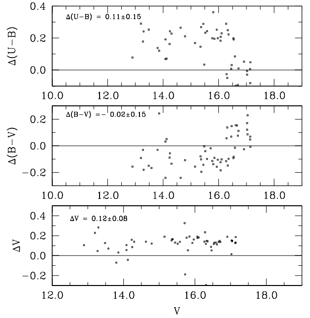
Fig. 3. Comparisons of the photometry presented in this paper with that of Moffat et al. (1991).
