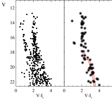
Fig. 10. Left panel , VI_c data for stars within 1.2' of the cluster center. Right panel , X-ray ( Chandra ) cleaned data for that same area reveals the cluster's main-sequence and pre-main-sequence populations. A Siess et al. (2000) \tau = 1.5 \times 10^6 yr isochrone was applied using the parameters established in Sect. 3.
