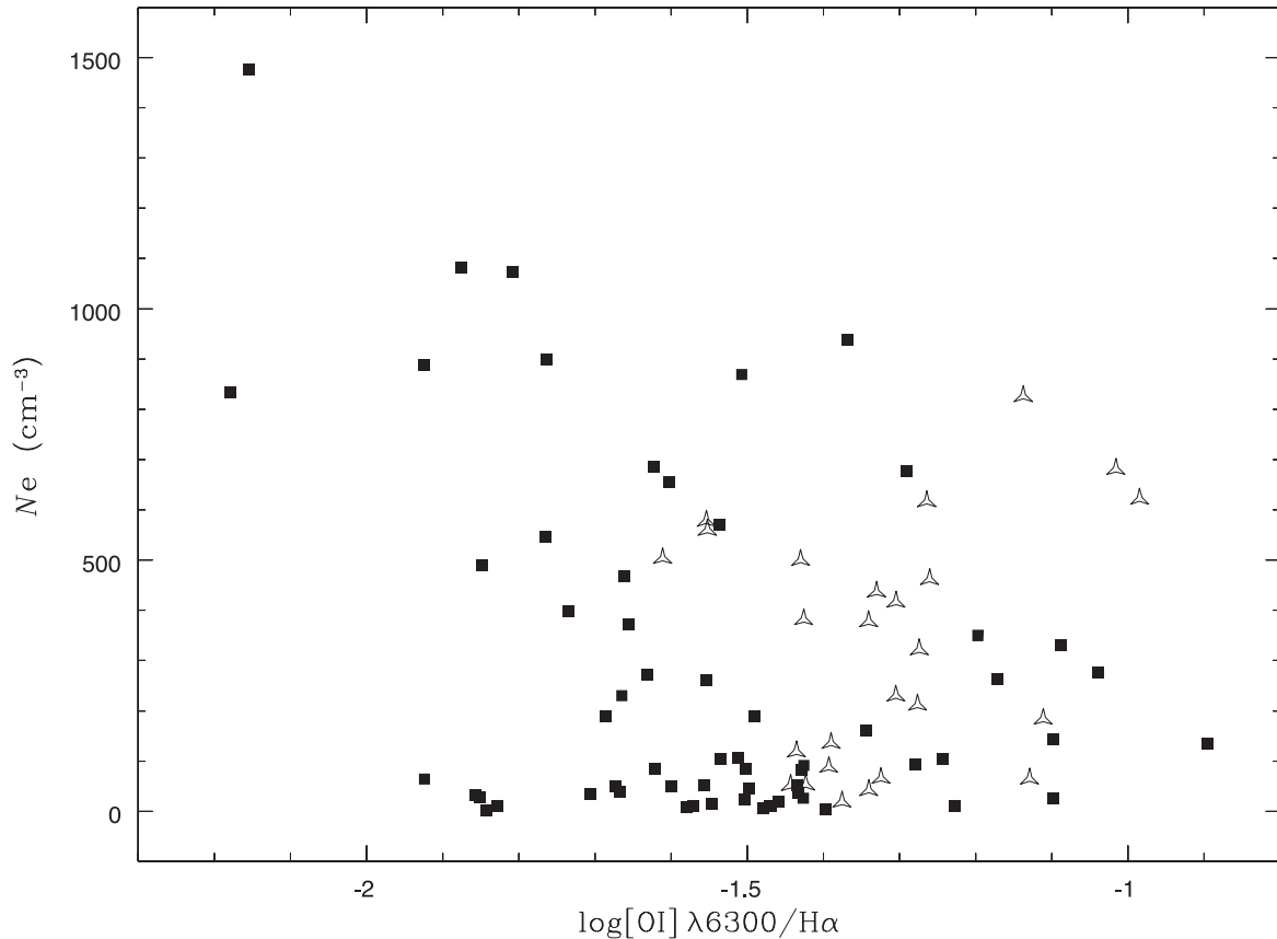
Figure 18. Electron density values N_e derived for our sample versus the observed [\text{O I}] \lambda 6300/\text{H}\alpha ratio. The squares represent regions ionized by massive stars while the triangles represent those with gas shock excitation, according to the diagnostic diagram presented in Fig. 17.
