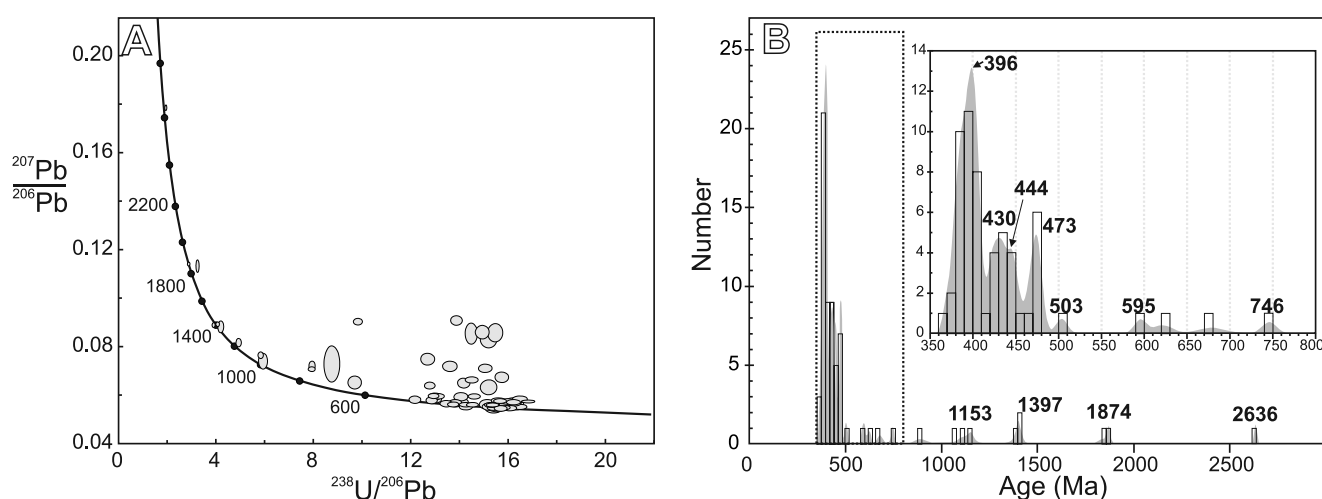
FIGURE 6. A) Tera-Wasserburg U-Pb Concordia diagrams for SHRIMP analyses from Cerro Negro basement sample zircons. B) Detrital zircon age distribution pattern (relative probability) for Cerro Negro basement sample.
