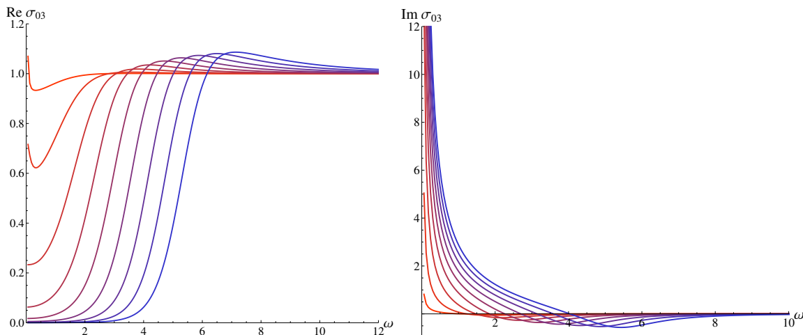
Figure 7. Plots of the Real (left) and Imaginary (right) parts of the conductivity for fixed S_x/\mu = 0.05 . Different lines correspond to different temperatures from T = 0.99T_c (red) to T = 0.38T_c (blue).
