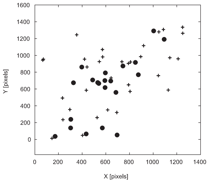
Fig. 7. The distribution of members (filled circles) and probable pre main sequence stars (crosses) in the area of Stock 16. The scale is the same used in Fig. 1.
