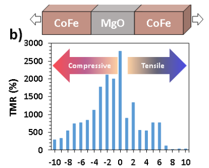
Fig. 8. a) Illustration of the hydrostatic deformations used to compute the TMR in epitaxial pMTJ stack. b) Resulting TMR obtained using DFT as a function of the strain applied in the pMTJ for an ideal CoFe|MgO|CoFe interface.
