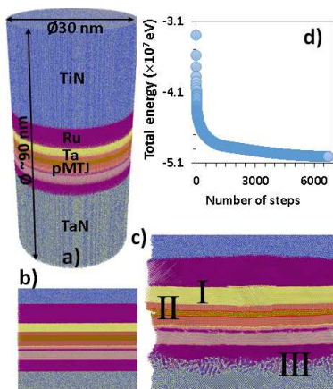
Fig. 6. Unrelaxed structure of the full STT-MRAM 30 nm diameter device (a). Transversal slice and zoomed view of stack before (b) and after (c) an atomic relaxation and the corresponding total energy minimization as a function of number numerical steps (d). I corresponds to the interface roughness, II to the MgO lift-off and III to Ru-TaN in-diffusion.
