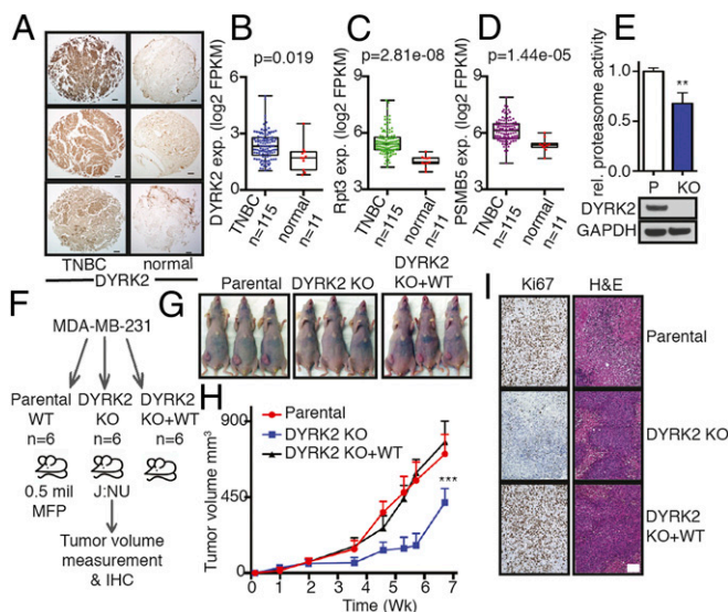
Fig. 1. DYRK2 and proteasome are up-regulated in TNBC and promote tumor progression. (A) DYRK2 IHC of TNBC and adjacent normal breast tissue sections from patients. (Scale bar, 100 \mu\text{m} .) (B) DYRK2, (C) RPT3, and (D) PSMB5 differential gene expression in human TNBC and matched normal tissue as available from TCGA (TNBC vs. normal tissue, P value derived from a semipaired modification to the Student's t test) (see also SI Appendix, Fig. S1). (E) Proteasome was affinity-purified from 1 mg of cell lysate of parental or DYRK2 KO MDA-MB-468 Rpn11-TBHA cells. Proteasome activity was measured with Suc-LLVY-AMC. **P < 0.01 (parental vs. DYRK2 KO, unpaired Student's t test, mean \pm SD from n = 3 independent experiments). Immunoblotting of the cell lysates were carried out with indicated antibodies. (F) Experimental flow for TNBC xenograft study in G–I. (G and H) MDA-MB-231 parental or DYRK2 KO or DYRK2 KO + WT rescue cells were injected into the mammary fat pad of J:NU nude mice. Tumor volume was measured twice a week ( n = 6 mice per condition), and growth curves were plotted. ***P < 0.001 (compared to parental group, 2-way ANOVA, mean \pm SD with Tukey's multiple comparison). (I) Histological examination of consecutive sections of the tumors (from G and H) with Ki67 and hematoxylin/eosin staining. (Scale bar, 100 \mu\text{m} .)
