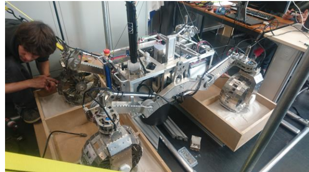
Figure 15: Partial gravity drilling test
