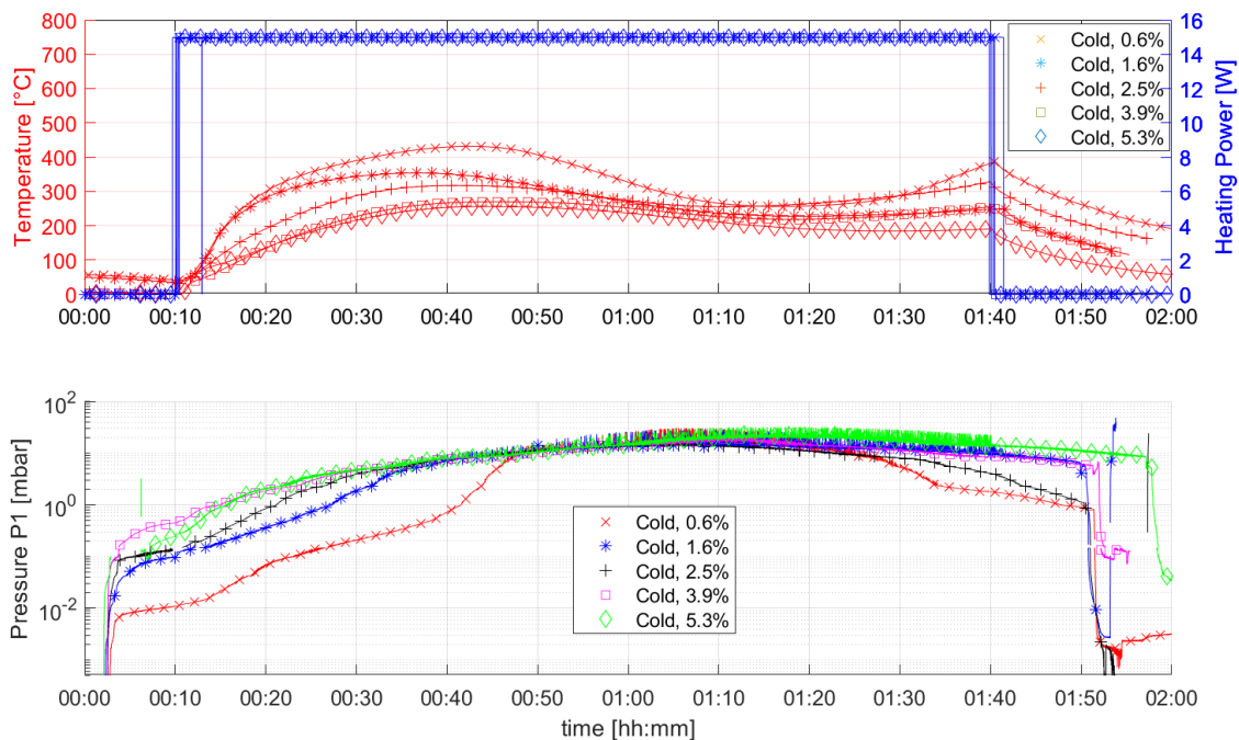
Figure 7: Gas extraction results with the VS and various water contents
