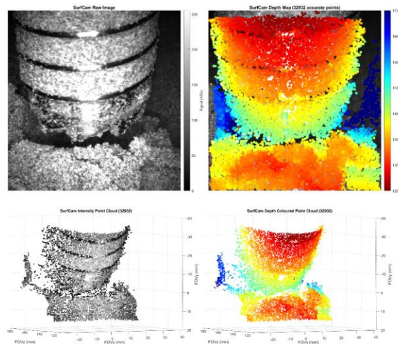
Figure 13: SurfCam image example during drilling
