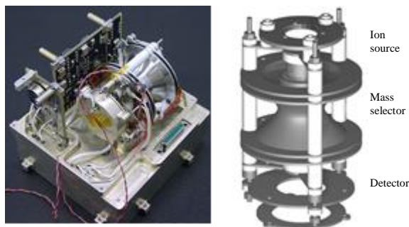
Figure 4: (Left) The Ptolemy ITMS with a mass range: 10 - 150 amu, resolution: 1 amu, mass: 500
