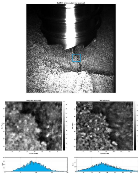
Figure 14: SurfCam super-resolution example immediately prior to drilling
