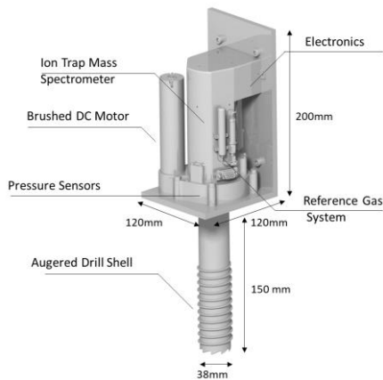
Figure 3: Render graphic and image of the Volatiles Sampler/Volatiles Analyser instrument
