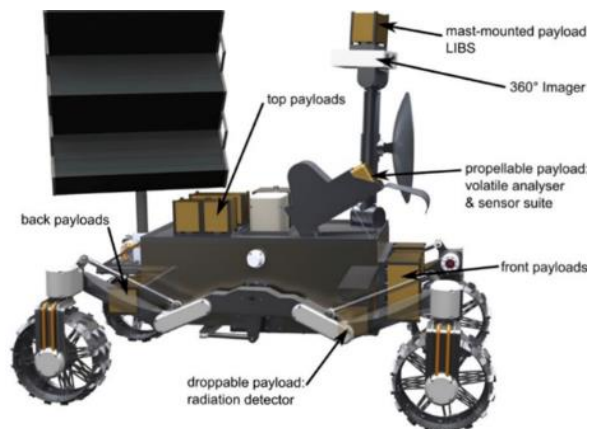
Figure 18: LUVMI-X notional concept
