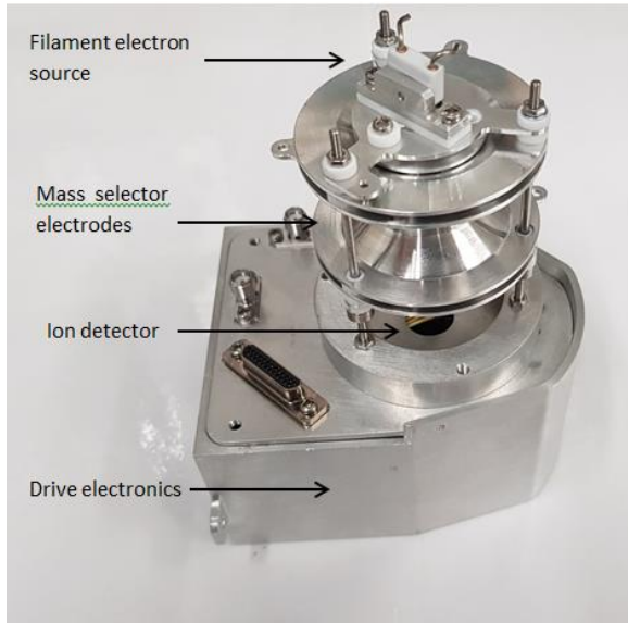
Figure 8: Image of the LUVMI VA ion trap mass spectrometer unit. mass: 700 gram, power: 8 W, dimensions approx. 13x10x10 cm.
