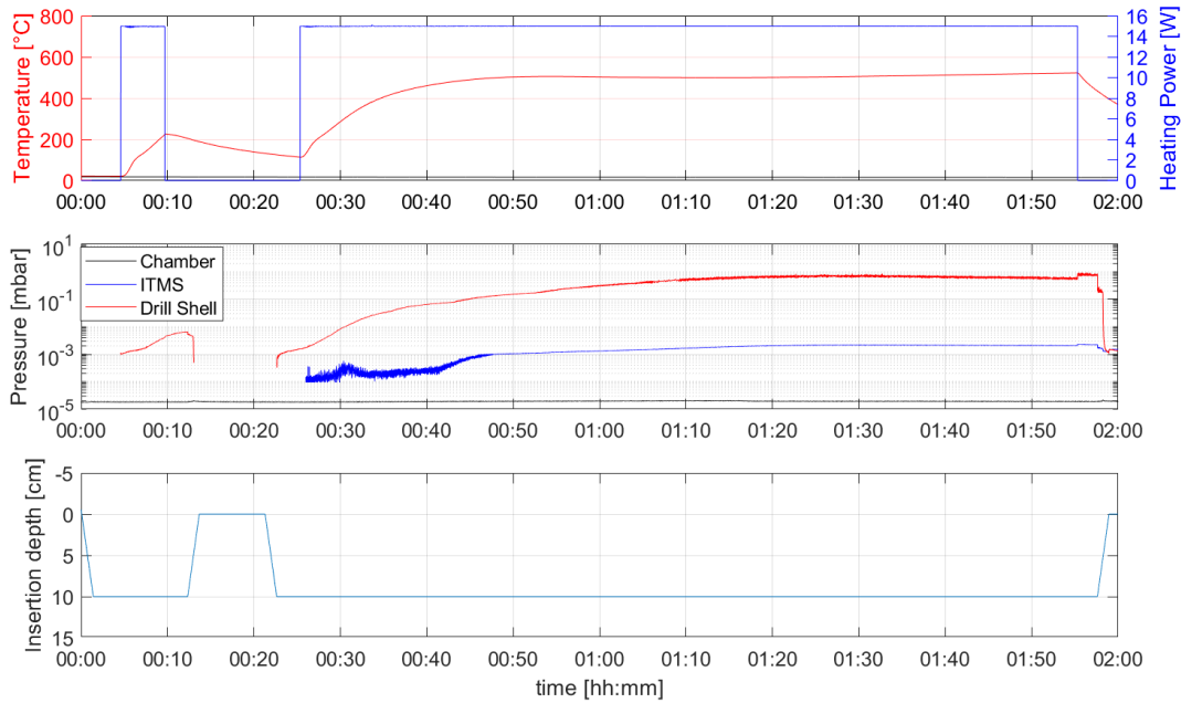
Figure 11: Gas extraction results of the integrated VS/VA test. Top Plot: Heater temperature and heating power; Center plot: Pressures of vacuum chamber, drill shell and VA volume; Lower Plot: Depth of insertion into regolith.
