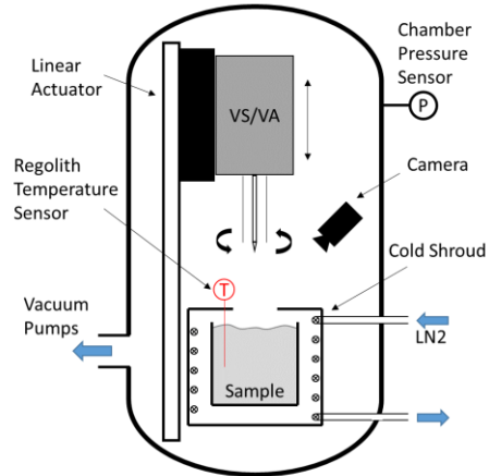
Figure 6: Schematic of the VS/VA test chamber
