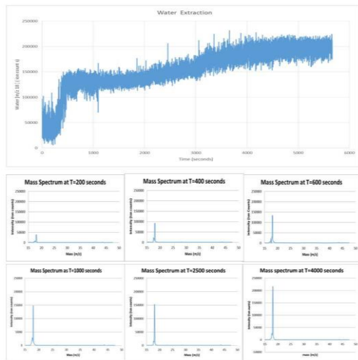
Figure 12: (top) showing the profile of m/z=18 (water) extracted from the simulant material during the 90 extraction experiment. The six individual mass spectra show increase in measured m/z 18 as the experiment progressed.
