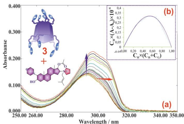
Fig. 2 a) UV-vis spectra of mixtures of pillar[5]arene 3 ( 10^{-5} M) with different concentrations of rocuronium bromide; b) Job's plot for the complex of rocuronium bromide with 3 .
