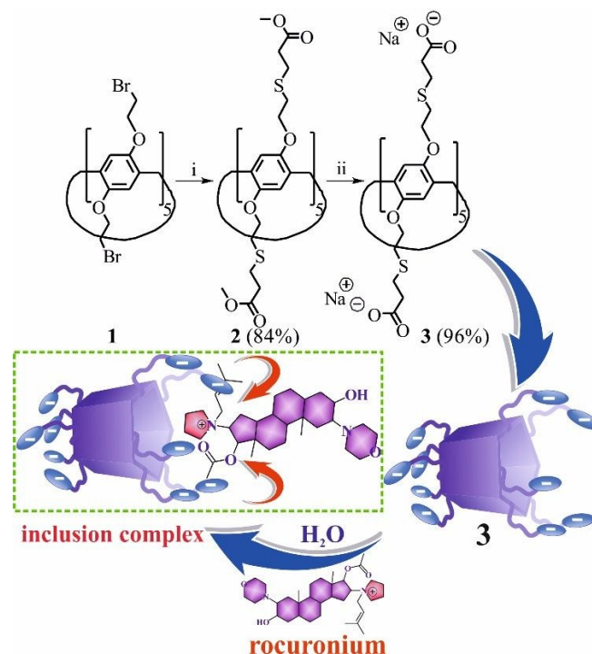
Fig. 1 Synthesis of macrocycles 2 and 3 ; the sketch represents the host-guest system of the 3 / rocuronium bromide. Reagents and conditions: i - methyl 3-mercaptopropionate, K_2CO_3 , DMF, r.t., 48h; ii - NaOH / H_2O / CH_3CH(OH)CH_3 , r.t., 4h.
