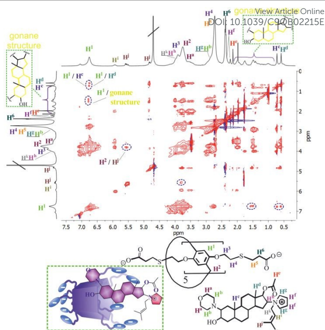
Fig. 5 The 2D ^1\text{H} - ^1\text{H} NOESY NMR spectrum of the 3 / rocuronium bromide complex (1:1, 1 \times 10^{-2} M) in \text{D}_2\text{O} at 25^\circ\text{C} and the proposed structure of the complex.
