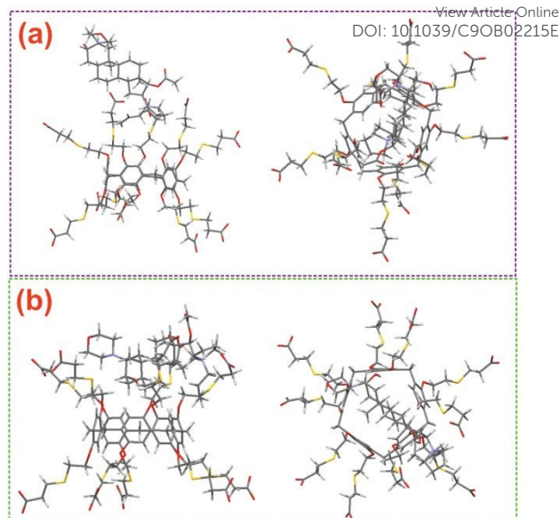
Fig. 6 Two calculated variants of orientation of the complex: with either (a) the pyrrolidine group or (b) the morpholine group oriented towards the macrocyclic annulus.
