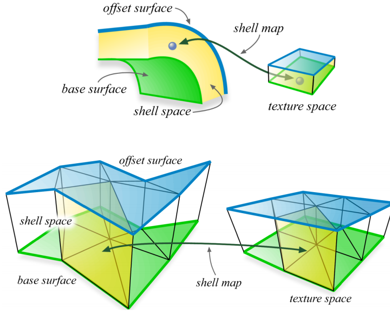
Figure 4. With shell mapping, 3D texture detail is mapped inside a thick layer over the surface of a model. Figures from [Porumbescu et al. 2005].
