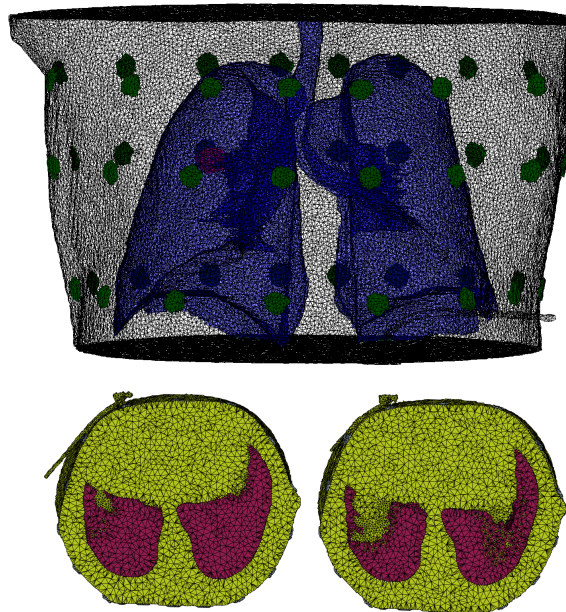
Figure 2: Fine FEM meshes of the human thorax. The top mesh shows the full mesh for the end inspiration instant. It contains 3 rings of 16 electrodes located two of them around the extremas of the lungs and the middle one in the tumour plane. The bottom meshes show the lowest electrode ring plane for end inspiration and end expiration.
