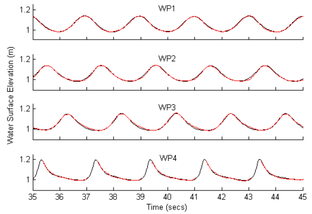
Figure 8 Time-series showing free-surface elevation measured at four cross-shore locations by both the LiDAR (red) and capacitance wave probes (black) during a ten second period. Note that the wave probe (WP) numbers refer to the positions defined in Figure 4.
